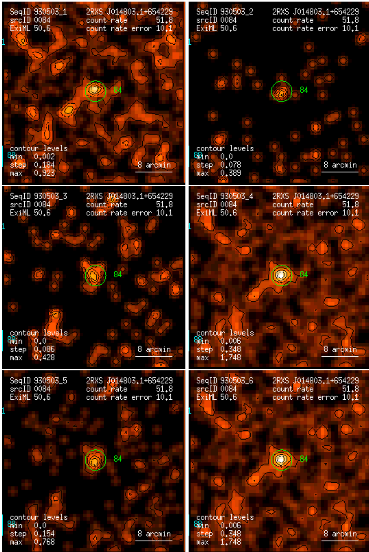
Figure 84: RASS 930503: detection 0084: band rate images, Gaussian filter: (1) PSPC channels 11 – 41, (2) 52 – 90, (3) 91 – 201, (4) 11 – 235, (5) 52 – 201, (6) 11 – 201. Broad band rates in counts/ks. Band rate contour levels in counts/ks/arcmin 2 .
