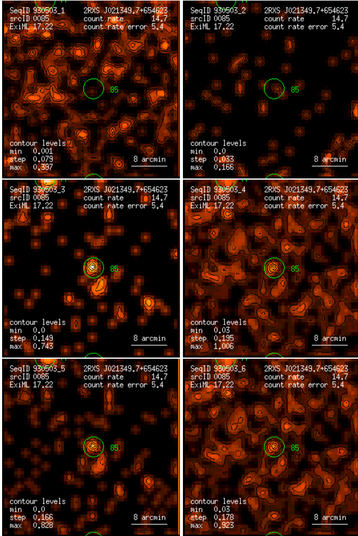
Figure 85: RASS 930503: detection 0085: band rate images, Gaussian filter: (1) PSPC channels 11 – 41, (2) 52 – 90, (3) 91 – 201, (4) 11 – 235, (5) 52 – 201, (6) 11 – 201. Broad band rates in counts/ks. Band rate contour levels in counts/ks/arcmin 2 .
