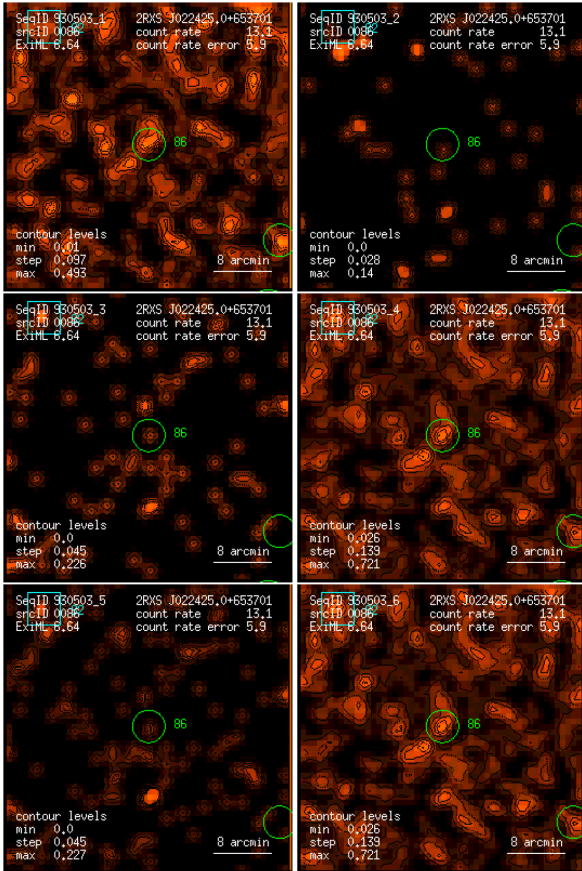
Figure 86: RASS 930503: detection 0086: band rate images, Gaussian filter: (1) PSPC channels 11 – 41, (2) 52 – 90, (3) 91 – 201, (4) 11 – 235, (5) 52 – 201, (6) 11 – 201. Broad band rates in counts/ks. Band rate contour levels in counts/ks/arcmin 2 .
