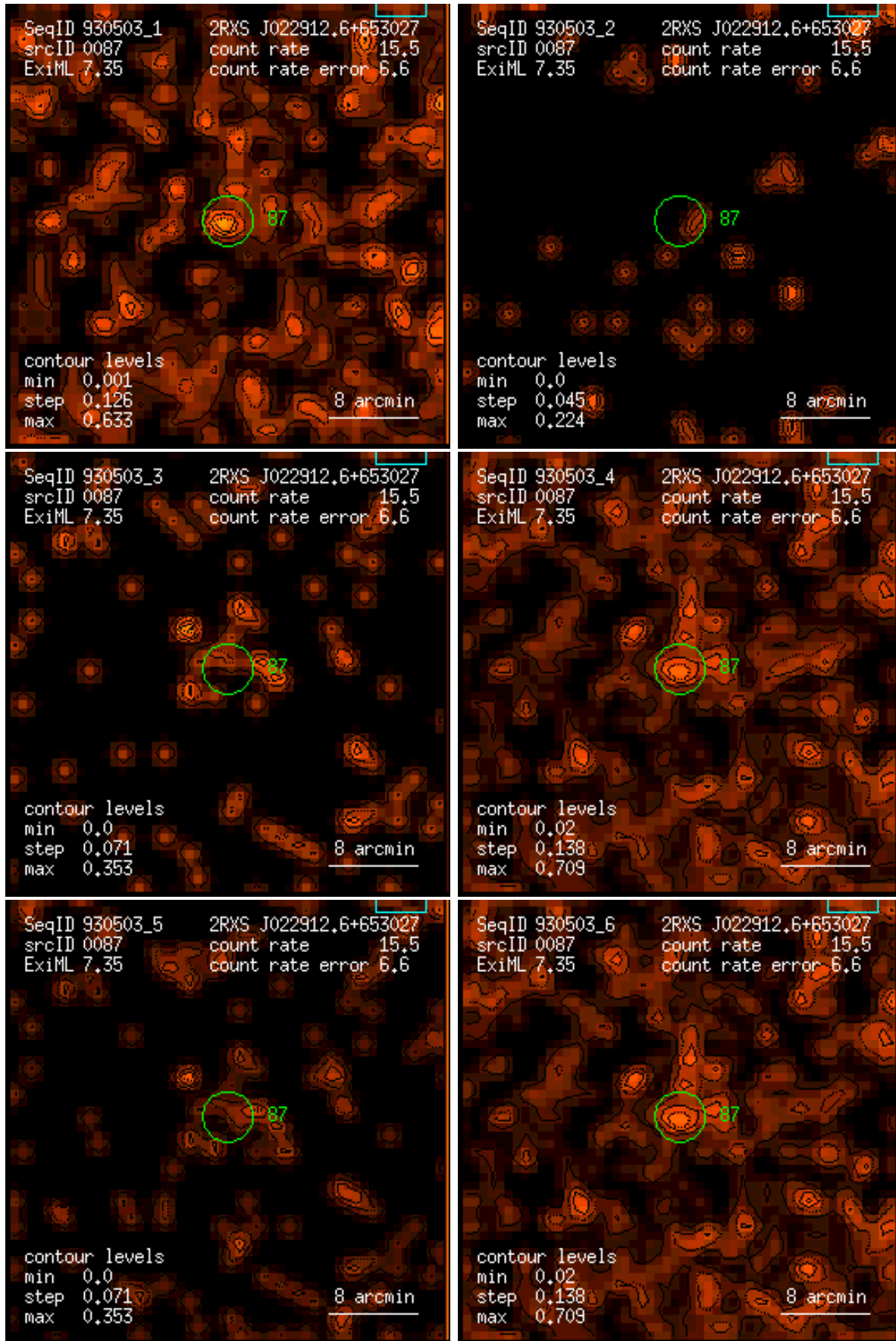
Figure 87: RASS 930503: detection 0087: band rate images, Gaussian filter: (1) PSPC channels 11 – 41, (2) 52 – 90, (3) 91 – 201, (4) 11 – 235, (5) 52 – 201, (6) 11 – 201. Broad band rates in counts/ks. Band rate contour levels in counts/ks/arcmin 2 .
