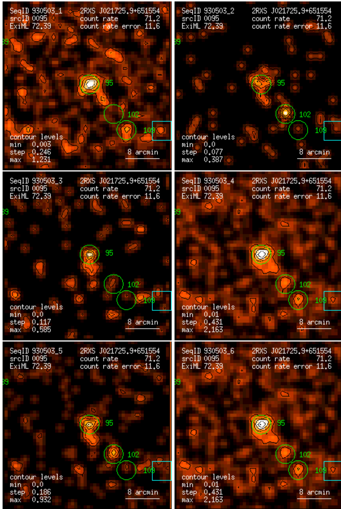
Figure 95: RASS 930503: detection 0095: band rate images, Gaussian filter: (1) PSPC channels 11 – 41, (2) 52 – 90, (3) 91 – 201, (4) 11 – 235, (5) 52 – 201, (6) 11 – 201. Broad band rates in counts/ks. Band rate contour levels in counts/ks/arcmin 2 .
