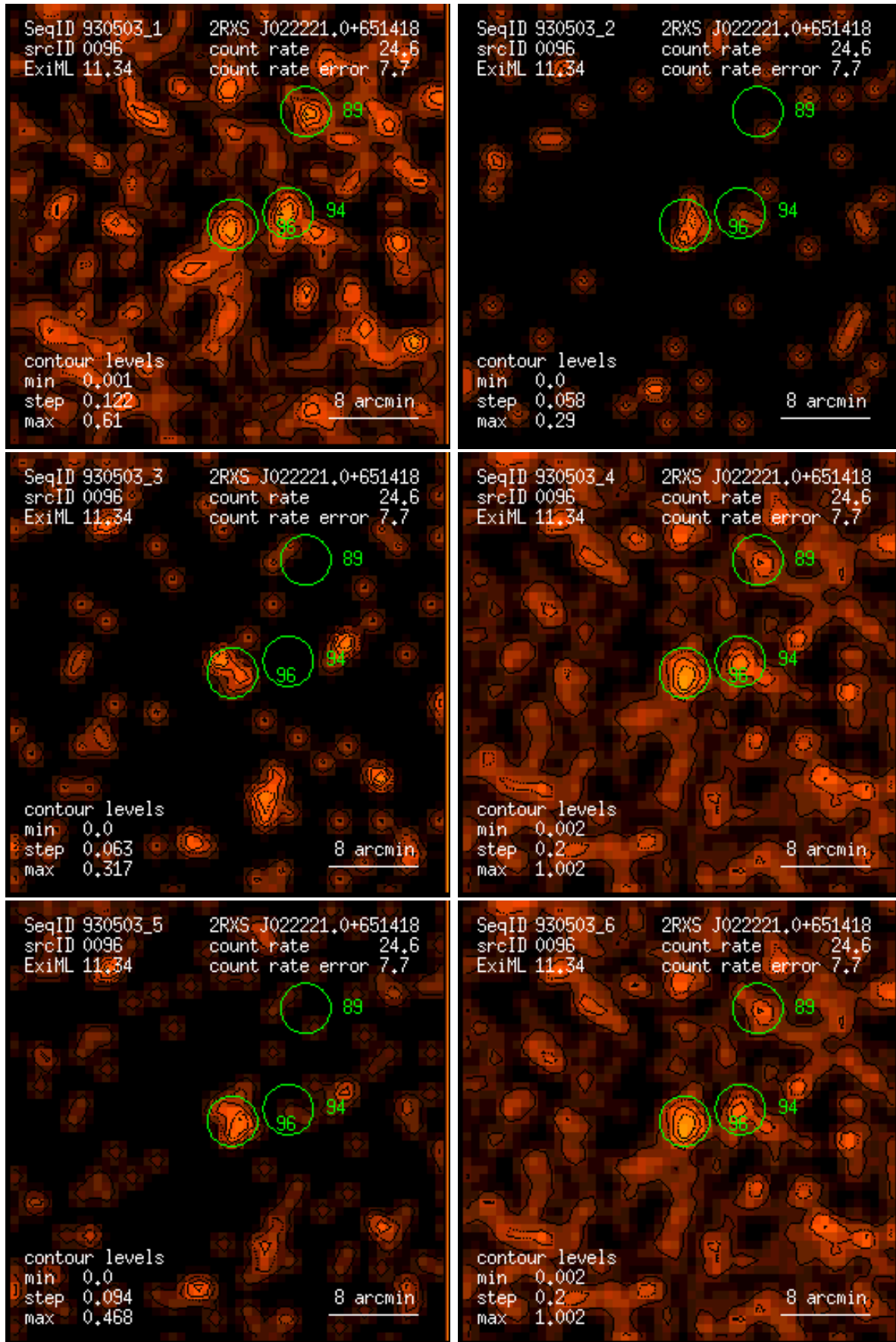
Figure 96: RASS 930503: detection 0096: band rate images, Gaussian filter: (1) PSPC channels 11 – 41, (2) 52 – 90, (3) 91 – 201, (4) 11 – 235, (5) 52 – 201, (6) 11 – 201. Broad band rates in counts/ks. Band rate contour levels in counts/ks/arcmin 2 .
