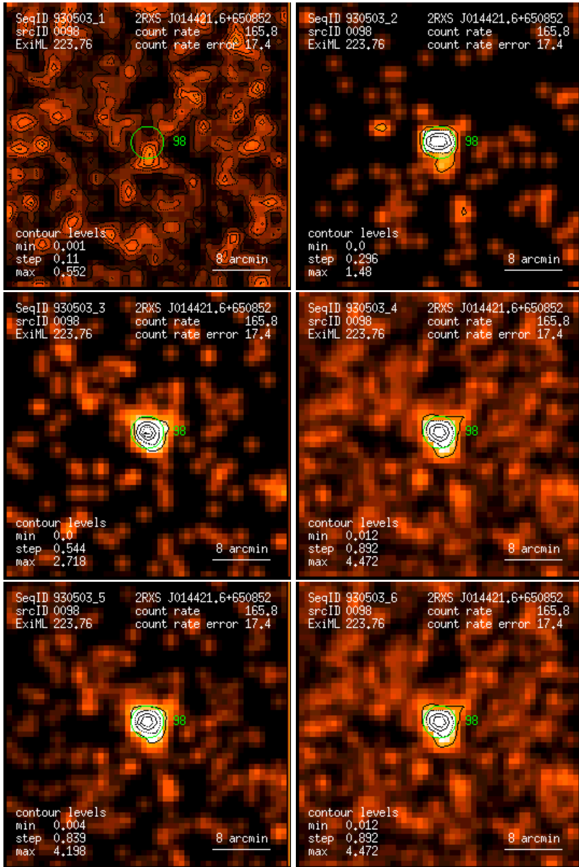
Figure 98: RASS 930503: detection 0098: band rate images, Gaussian filter: (1) PSPC channels 11 – 41, (2) 52 – 90, (3) 91 – 201, (4) 11 – 235, (5) 52 – 201, (6) 11 – 201. Broad band rates in counts/ks. Band rate contour levels in counts/ks/arcmin 2 .
