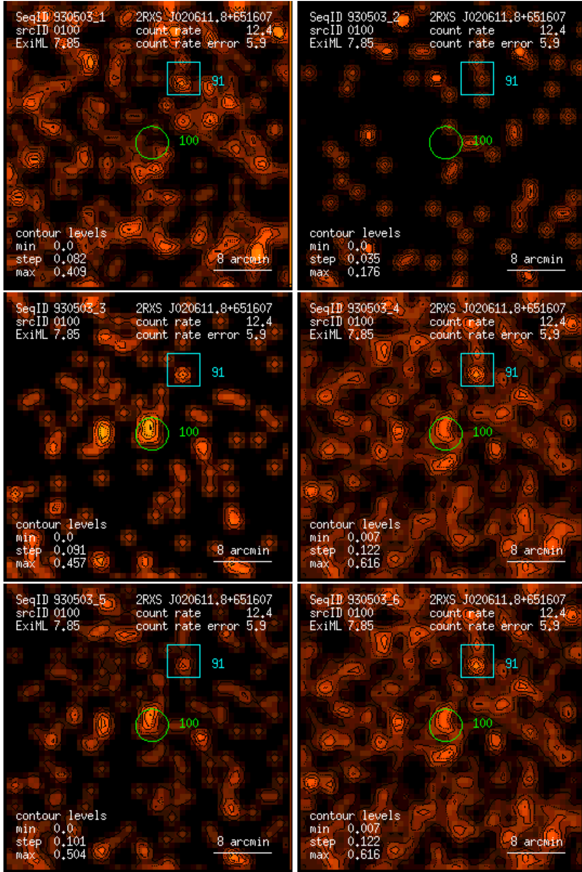
Figure 100: RASS 930503: detection 0100: band rate images, Gaussian filter: (1) PSPC channels 11 – 41, (2) 52 – 90, (3) 91 – 201, (4) 11 – 235, (5) 52 – 201, (6) 11 – 201. Broad band rates in counts/ks. Band rate contour levels in counts/ks/arcmin 2 .
