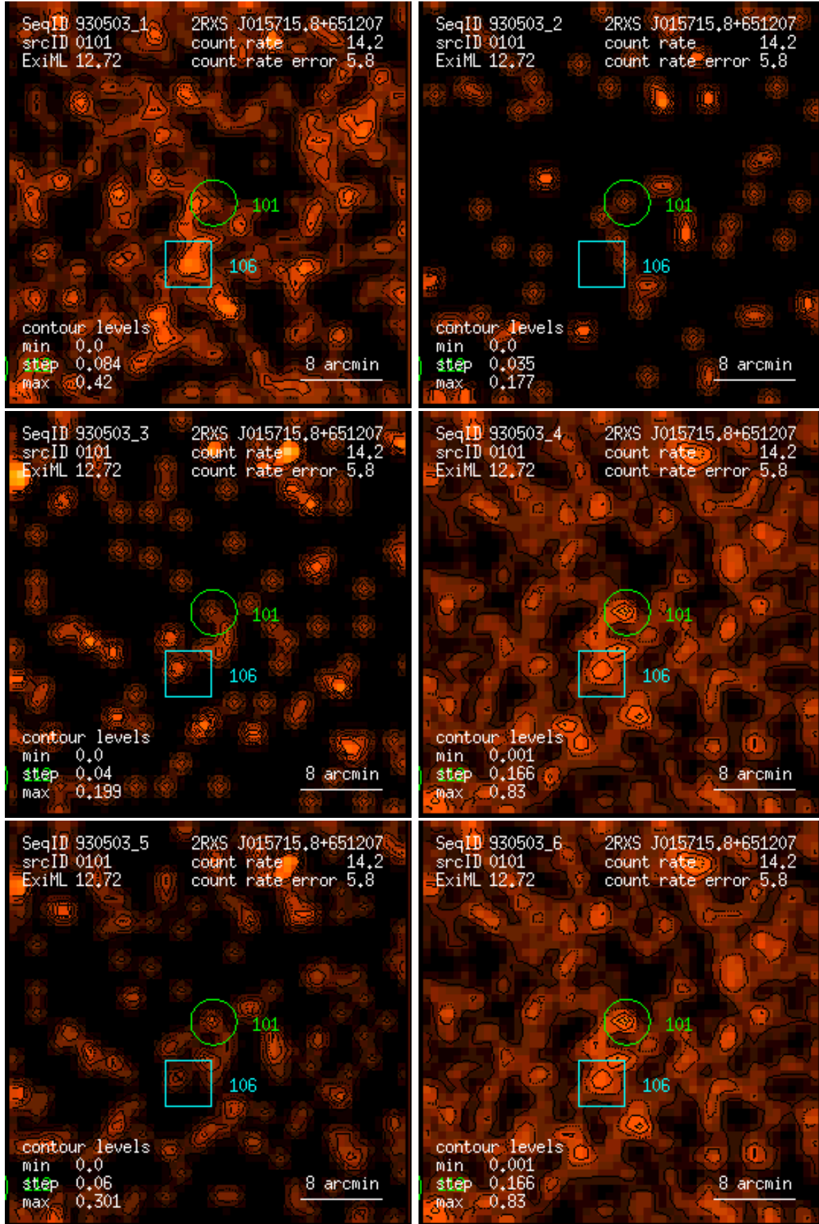
Figure 101: RASS 930503: detection 0101: band rate images, Gaussian filter: (1) PSPC channels 11 – 41, (2) 52 – 90, (3) 91 – 201, (4) 11 – 235, (5) 52 – 201, (6) 11 – 201. Broad band rates in counts/ks. Band rate contour levels in counts/ks/arcmin 2 .
