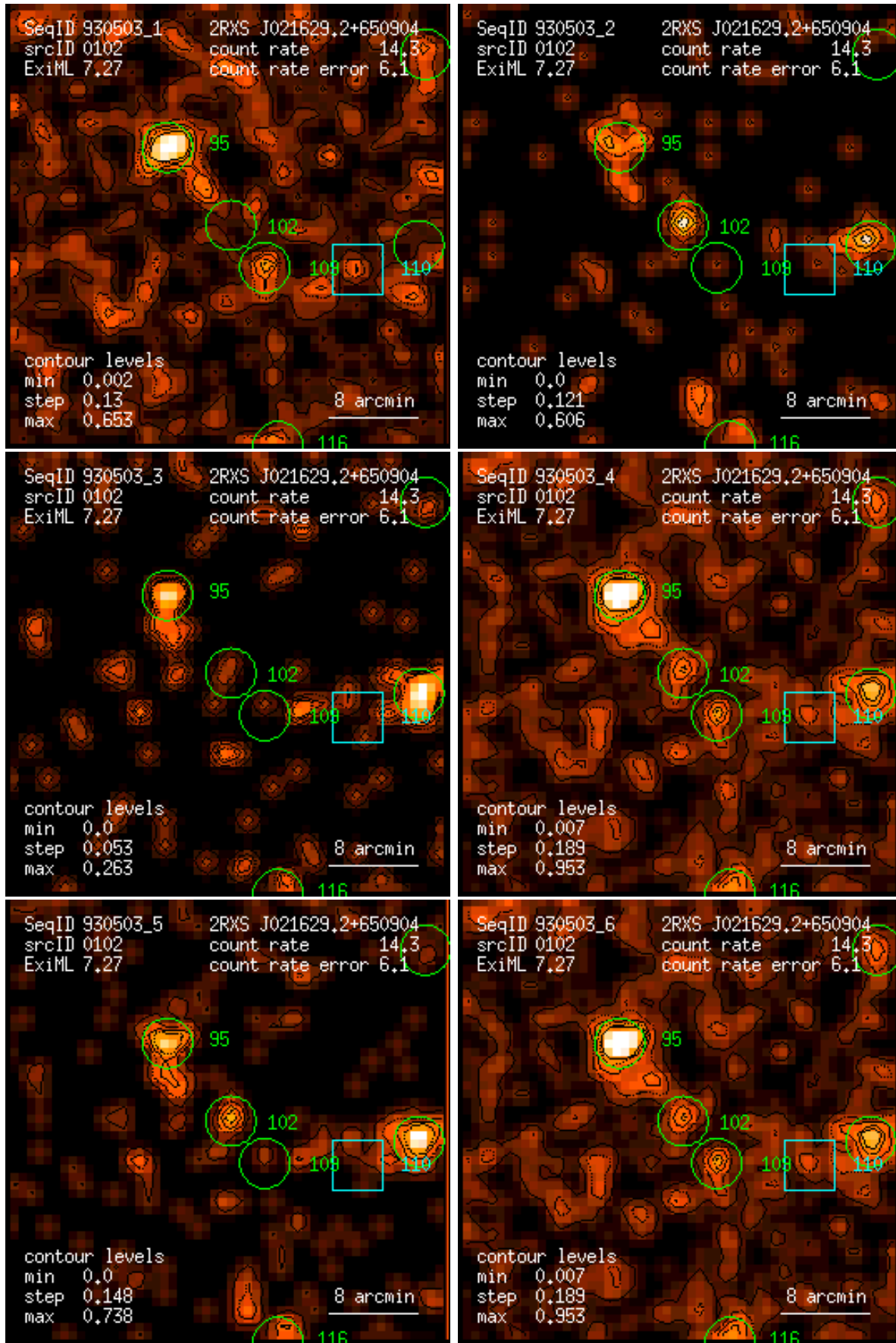
Figure 102: RASS 930503: detection 0102: band rate images, Gaussian filter: (1) PSPC channels 11 – 41, (2) 52 – 90, (3) 91 – 201, (4) 11 – 235, (5) 52 – 201, (6) 11 – 201. Broad band rates in counts/ks. Band rate contour levels in counts/ks/arcmin 2 .
