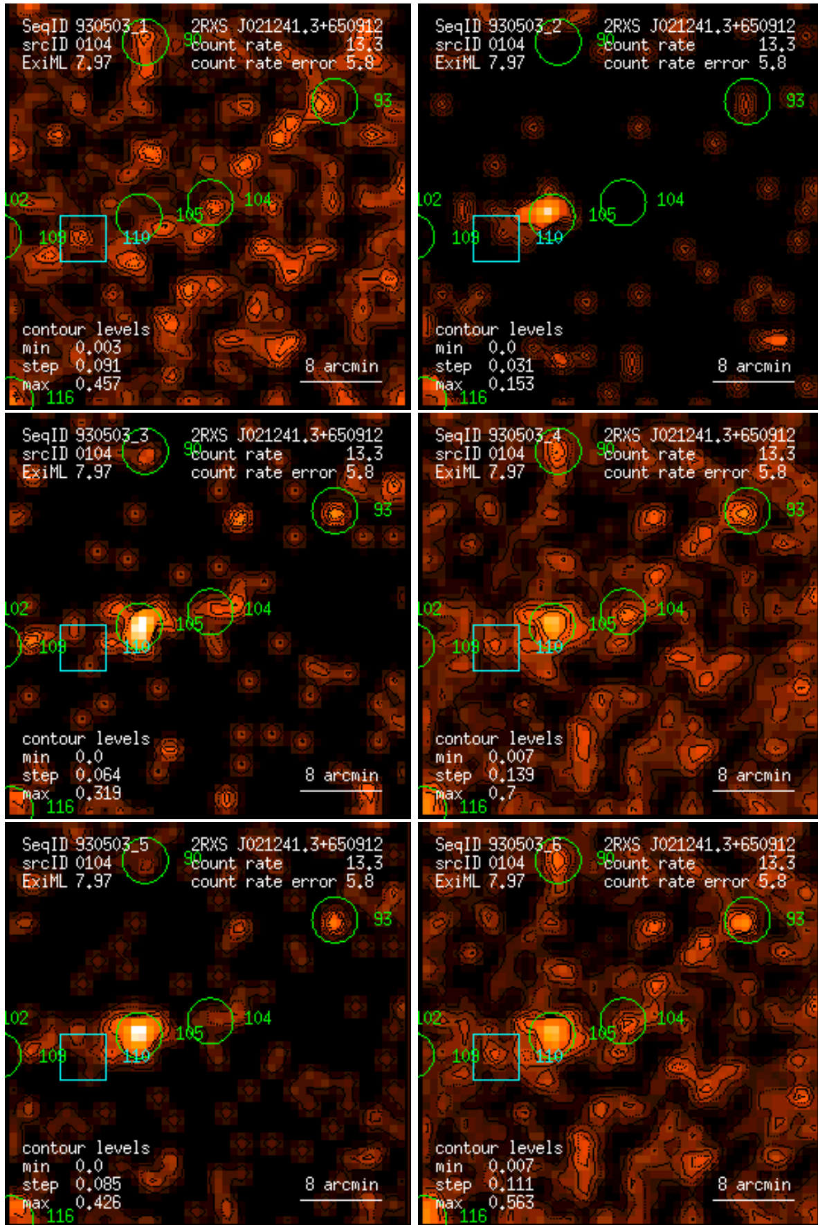
Figure 104: RASS 930503: detection 0104: band rate images, Gaussian filter: (1) PSPC channels 11 – 41, (2) 52 – 90, (3) 91 – 201, (4) 11 – 235, (5) 52 – 201, (6) 11 – 201. Broad band rates in counts/ks. Band rate contour levels in counts/ks/arcmin 2 .
