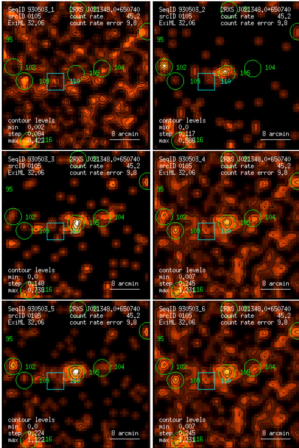
Figure 105: RASS 930503: detection 0105: band rate images, Gaussian filter: (1) PSPC channels 11 – 41, (2) 52 – 90, (3) 91 – 201, (4) 11 – 235, (5) 52 – 201, (6) 11 – 201. Broad band rates in counts/ks. Band rate contour levels in counts/ks/arcmin 2 .
