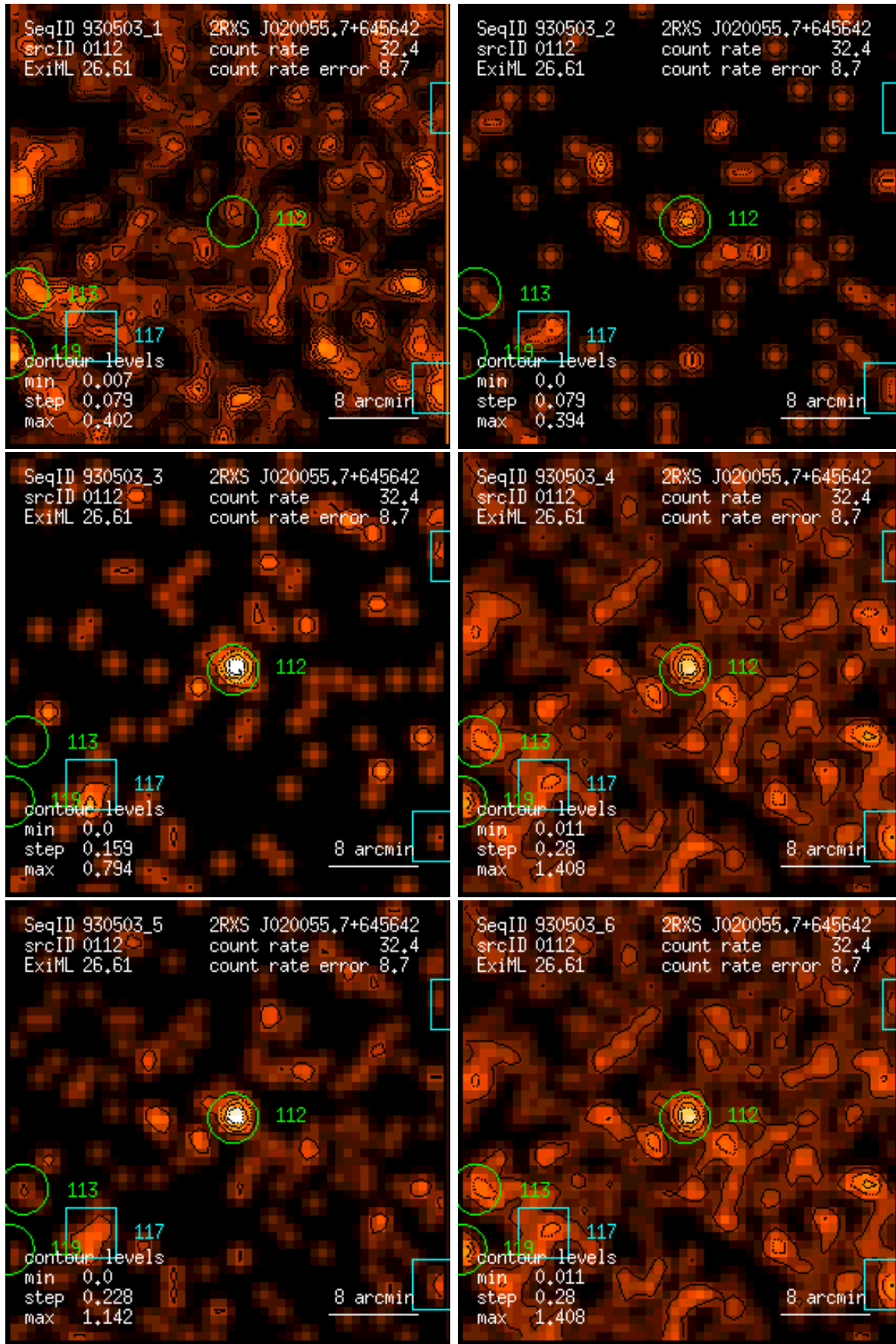
Figure 112: RASS 930503: detection 0112: band rate images, Gaussian filter: (1) PSPC channels 11 – 41, (2) 52 – 90, (3) 91 – 201, (4) 11 – 235, (5) 52 – 201, (6) 11 – 201. Broad band rates in counts/ks. Band rate contour levels in counts/ks/arcmin 2 .
