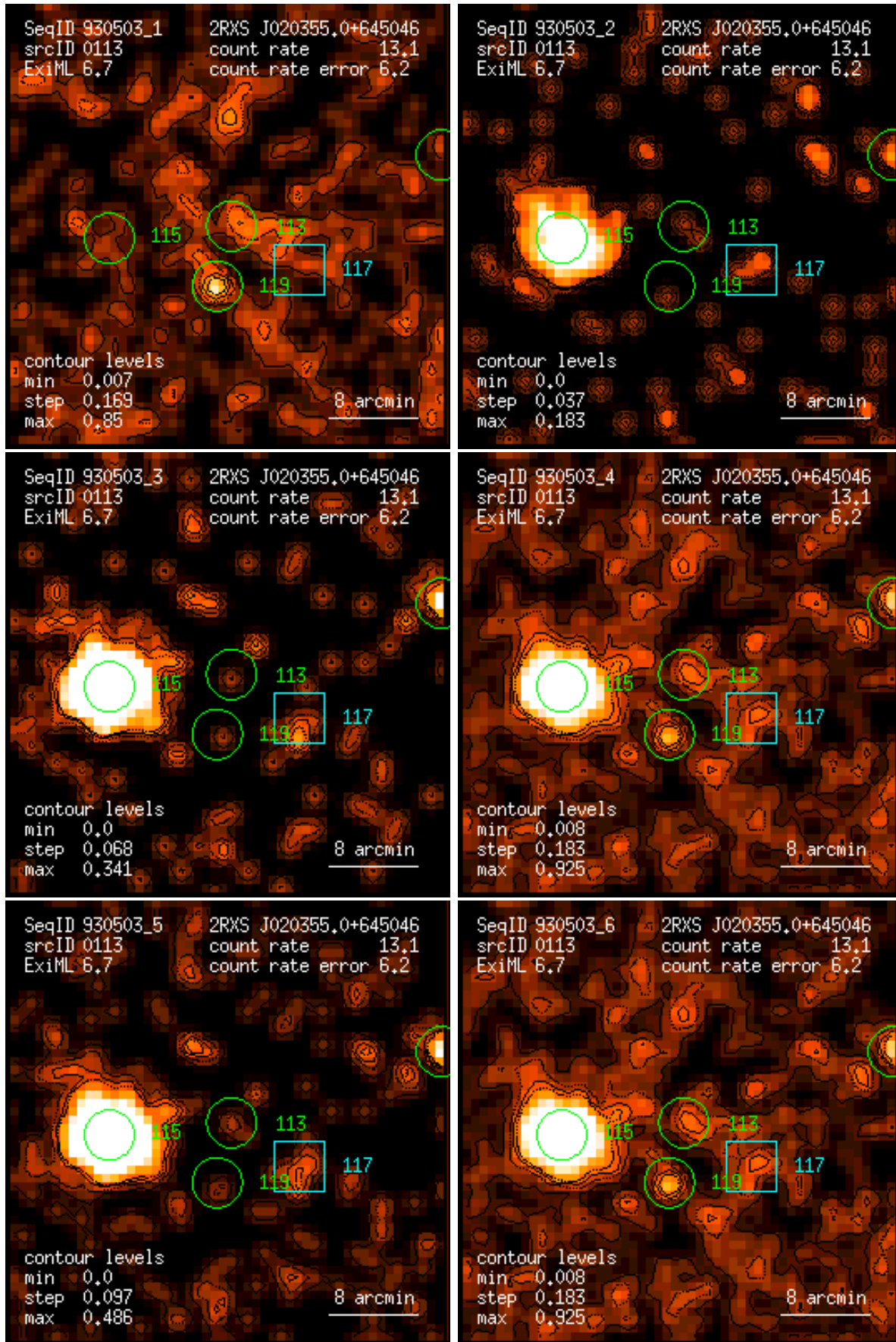
Figure 113: RASS 930503: detection 0113: band rate images, Gaussian filter: (1) PSPC channels 11 – 41, (2) 52 – 90, (3) 91 – 201, (4) 11 – 235, (5) 52 – 201, (6) 11 – 201. Broad band rates in counts/ks. Band rate contour levels in counts/ks/arcmin 2 .
