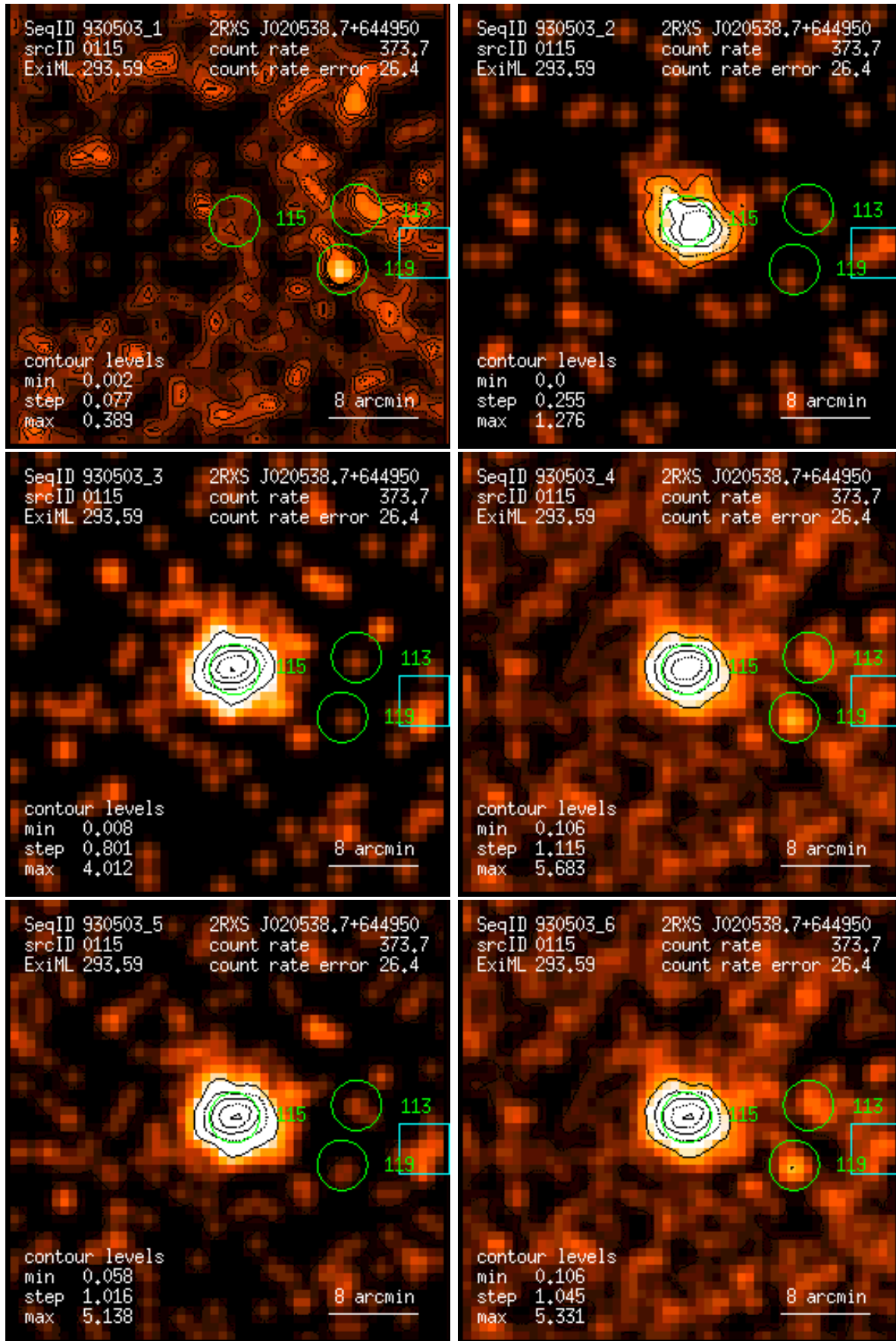
Figure 115: RASS 930503: detection 0115: band rate images, Gaussian filter: (1) PSPC channels 11 – 41, (2) 52 – 90, (3) 91 – 201, (4) 11 – 235, (5) 52 – 201, (6) 11 – 201. Broad band rates in counts/ks. Band rate contour levels in counts/ks/arcmin 2 .
