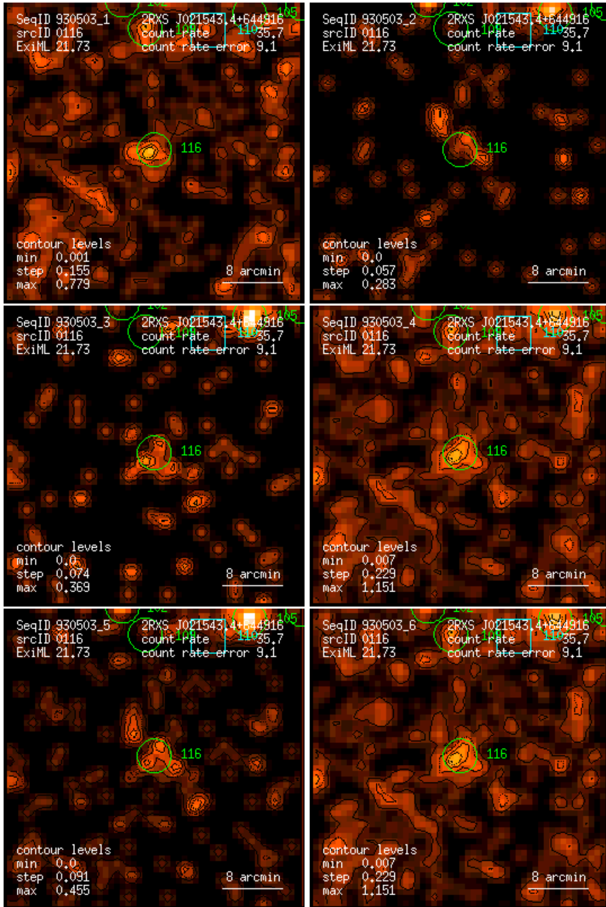
Figure 116: RASS 930503: detection 0116: band rate images, Gaussian filter: (1) PSPC channels 11 – 41, (2) 52 – 90, (3) 91 – 201, (4) 11 – 235, (5) 52 – 201, (6) 11 – 201. Broad band rates in counts/ks. Band rate contour levels in counts/ks/arcmin 2 .
