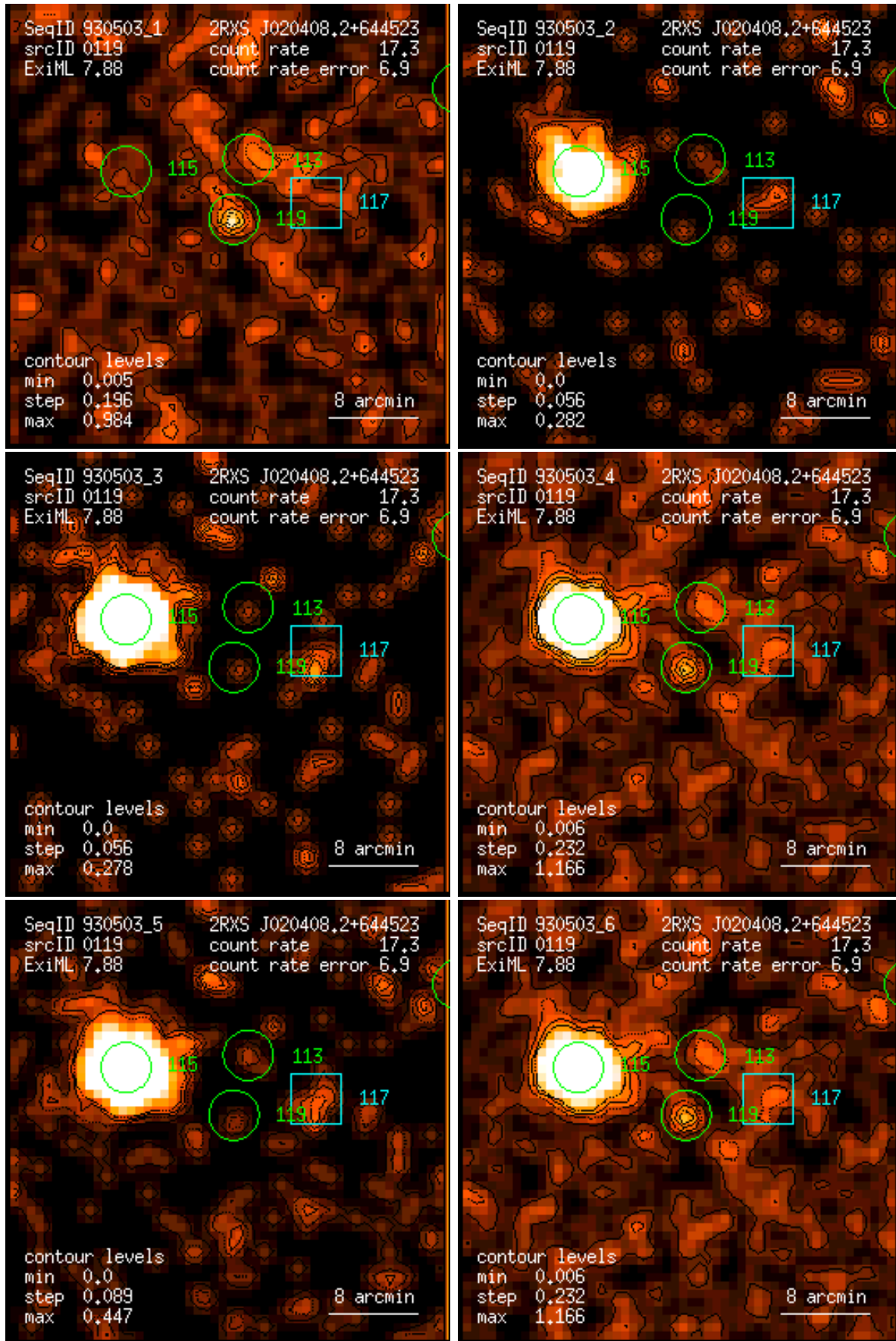
Figure 119: RASS 930503: detection 0119: band rate images, Gaussian filter: (1) PSPC channels 11 – 41, (2) 52 – 90, (3) 91 – 201, (4) 11 – 235, (5) 52 – 201, (6) 11 – 201. Broad band rates in counts/ks. Band rate contour levels in counts/ks/arcmin 2 .
