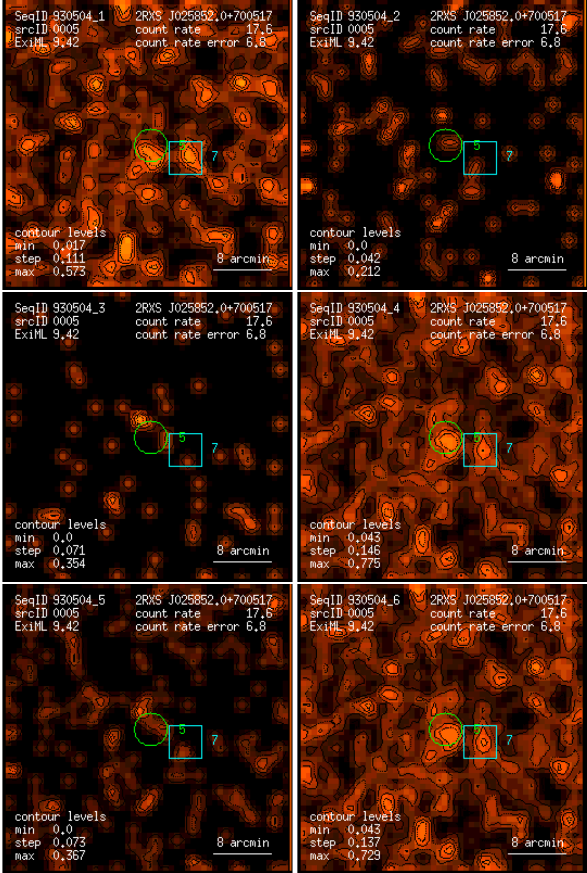
Figure 5: RASS 930504: detection 0005: band rate images, Gaussian filter: (1) PSPC channels 11 – 41, (2) 52 – 90, (3) 91 – 201, (4) 11 – 235, (5) 52 – 201, (6) 11 – 201. Broad band rates in counts/ks. Band rate contour levels in counts/ks/arcmin 2 .
