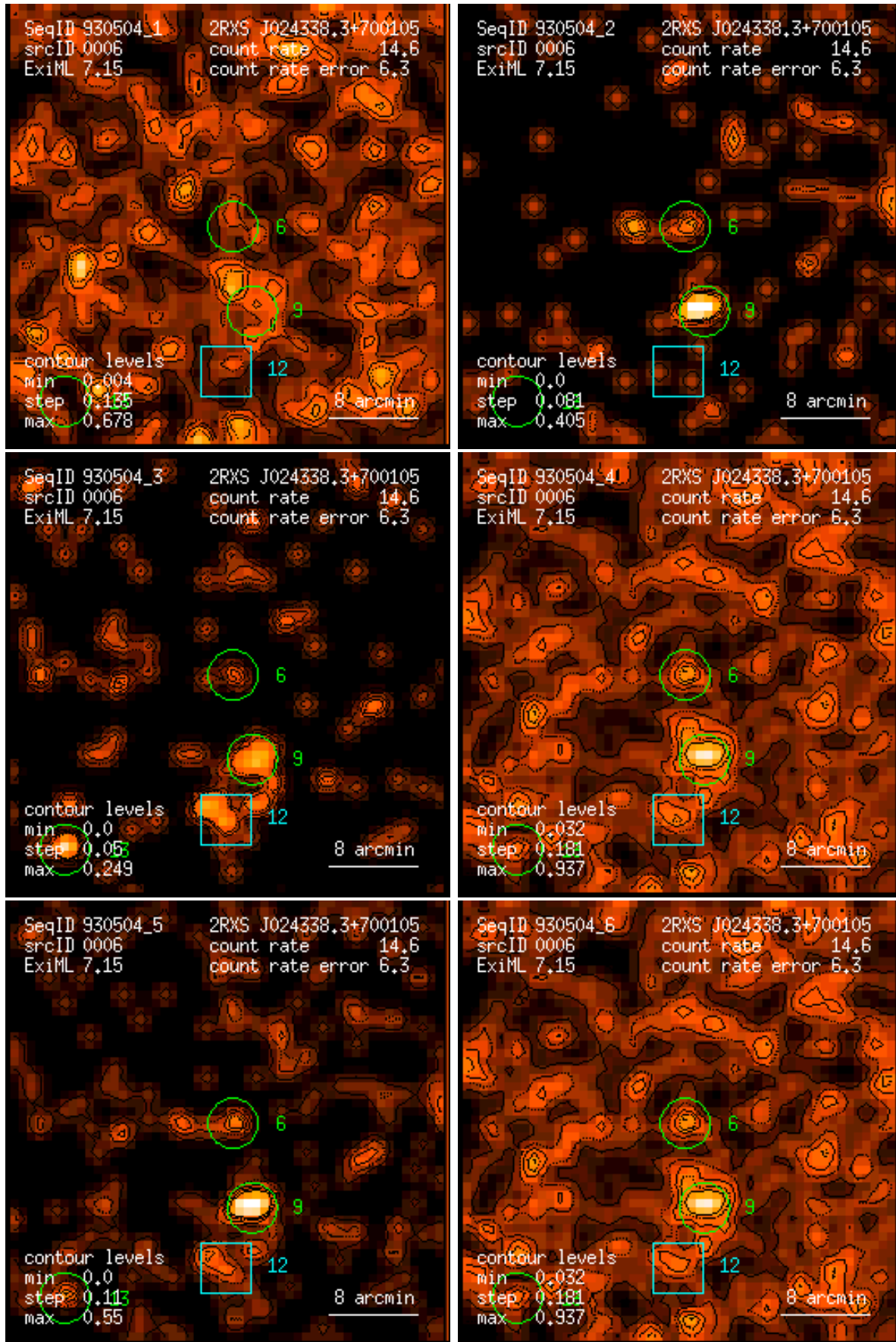
Figure 6: RASS 930504: detection 0006: band rate images, Gaussian filter: (1) PSPC channels 11 – 41, (2) 52 – 90, (3) 91 – 201, (4) 11 – 235, (5) 52 – 201, (6) 11 – 201. Broad band rates in counts/ks. Band rate contour levels in counts/ks/arcmin 2 .
