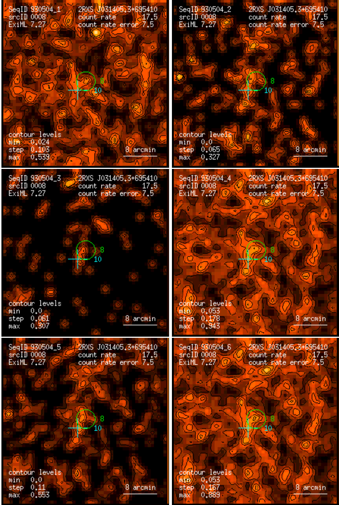
Figure 8: RASS 930504: detection 0008: band rate images, Gaussian filter: (1) PSPC channels 11 – 41, (2) 52 – 90, (3) 91 – 201, (4) 11 – 235, (5) 52 – 201, (6) 11 – 201. Broad band rates in counts/ks. Band rate contour levels in counts/ks/arcmin 2 .
