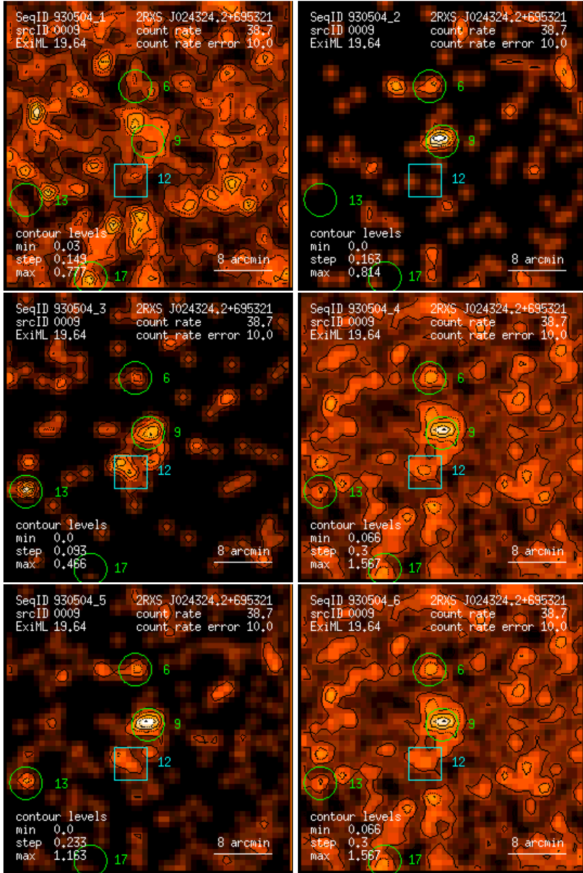
Figure 9: RASS 930504: detection 0009: band rate images, Gaussian filter: (1) PSPC channels 11 – 41, (2) 52 – 90, (3) 91 – 201, (4) 11 – 235, (5) 52 – 201, (6) 11 – 201. Broad band rates in counts/ks. Band rate contour levels in counts/ks/arcmin 2 .
