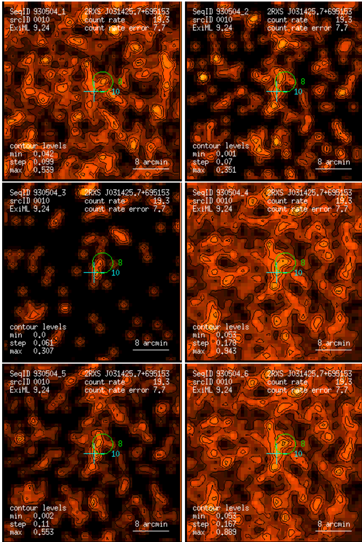
Figure 10: RASS 930504: detection 0010: band rate images, Gaussian filter: (1) PSPC channels 11 – 41, (2) 52 – 90, (3) 91 – 201, (4) 11 – 235, (5) 52 – 201, (6) 11 – 201. Broad band rates in counts/ks. Band rate contour levels in counts/ks/arcmin 2 .
