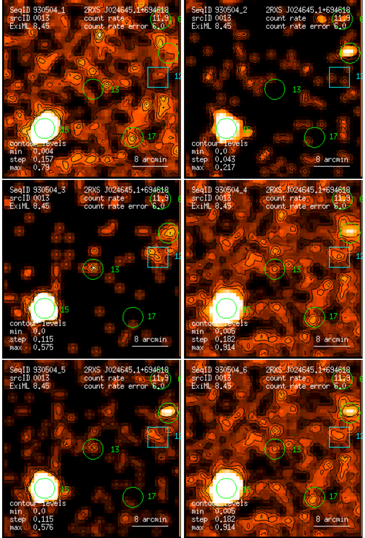
Figure 13: RASS 930504: detection 0013: band rate images, Gaussian filter: (1) PSPC channels 11 – 41, (2) 52 – 90, (3) 91 – 201, (4) 11 – 235, (5) 52 – 201, (6) 11 – 201. Broad band rates in counts/ks. Band rate contour levels in counts/ks/arcmin 2 .
