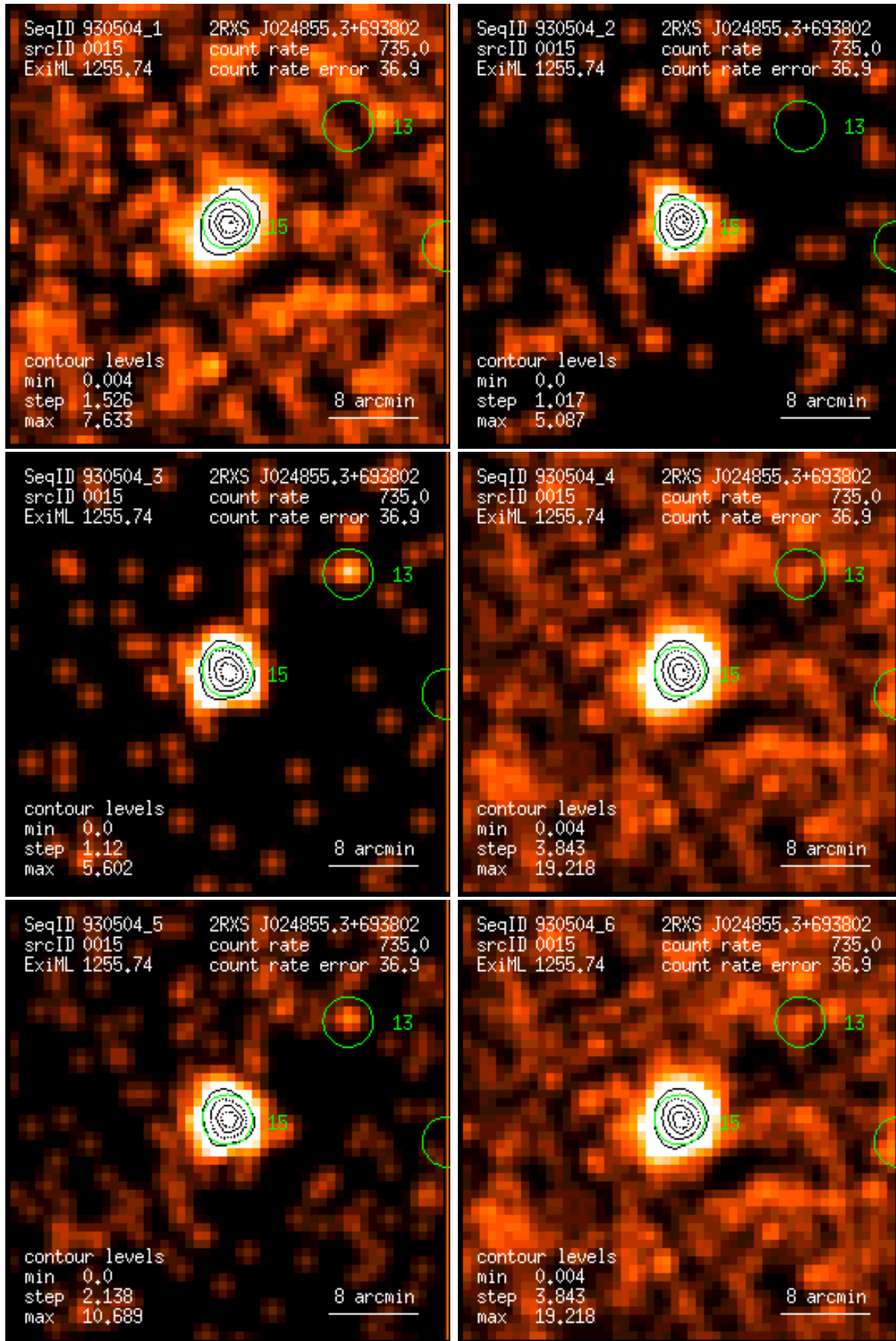
Figure 15: RASS 930504: detection 0015: band rate images, Gaussian filter: (1) PSPC channels 11 – 41, (2) 52 – 90, (3) 91 – 201, (4) 11 – 235, (5) 52 – 201, (6) 11 – 201. Broad band rates in counts/ks. Band rate contour levels in counts/ks/arcmin 2 .
