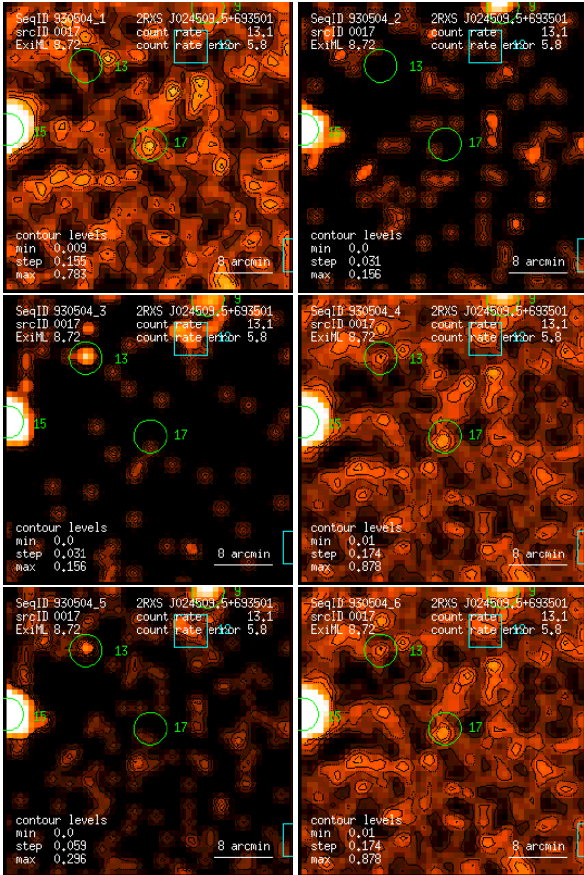
Figure 17: RASS 930504: detection 0017: band rate images, Gaussian filter: (1) PSPC channels 11 – 41, (2) 52 – 90, (3) 91 – 201, (4) 11 – 235, (5) 52 – 201, (6) 11 – 201. Broad band rates in counts/ks. Band rate contour levels in counts/ks/arcmin 2 .
