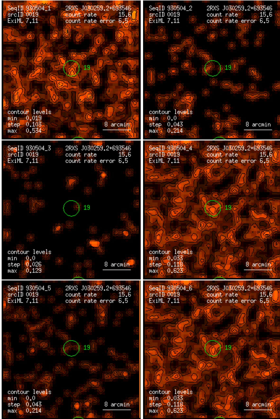
Figure 19: RASS 930504: detection 0019: band rate images, Gaussian filter: (1) PSPC channels 11 – 41, (2) 52 – 90, (3) 91 – 201, (4) 11 – 235, (5) 52 – 201, (6) 11 – 201. Broad band rates in counts/ks. Band rate contour levels in counts/ks/arcmin 2 .
