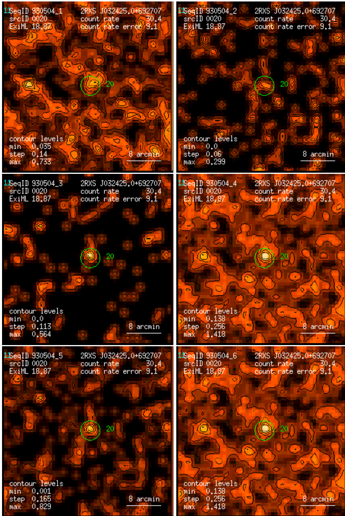
Figure 20: RASS 930504: detection 0020: band rate images, Gaussian filter: (1) PSPC channels 11 – 41, (2) 52 – 90, (3) 91 – 201, (4) 11 – 235, (5) 52 – 201, (6) 11 – 201. Broad band rates in counts/ks. Band rate contour levels in counts/ks/arcmin 2 .
