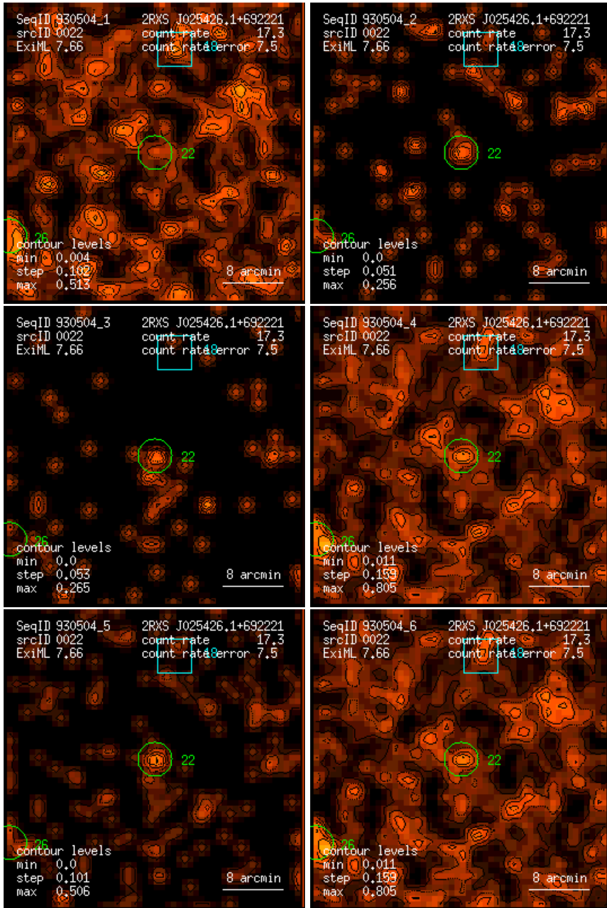
Figure 22: RASS 930504: detection 0022: band rate images, Gaussian filter: (1) PSPC channels 11 – 41, (2) 52 – 90, (3) 91 – 201, (4) 11 – 235, (5) 52 – 201, (6) 11 – 201. Broad band rates in counts/ks. Band rate contour levels in counts/ks/arcmin 2 .
