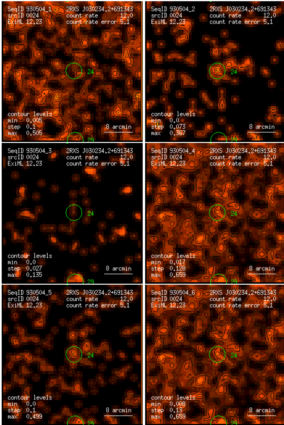
Figure 24: RASS 930504: detection 0024: band rate images, Gaussian filter: (1) PSPC channels 11 – 41, (2) 52 – 90, (3) 91 – 201, (4) 11 – 235, (5) 52 – 201, (6) 11 – 201. Broad band rates in counts/ks. Band rate contour levels in counts/ks/arcmin 2 .
