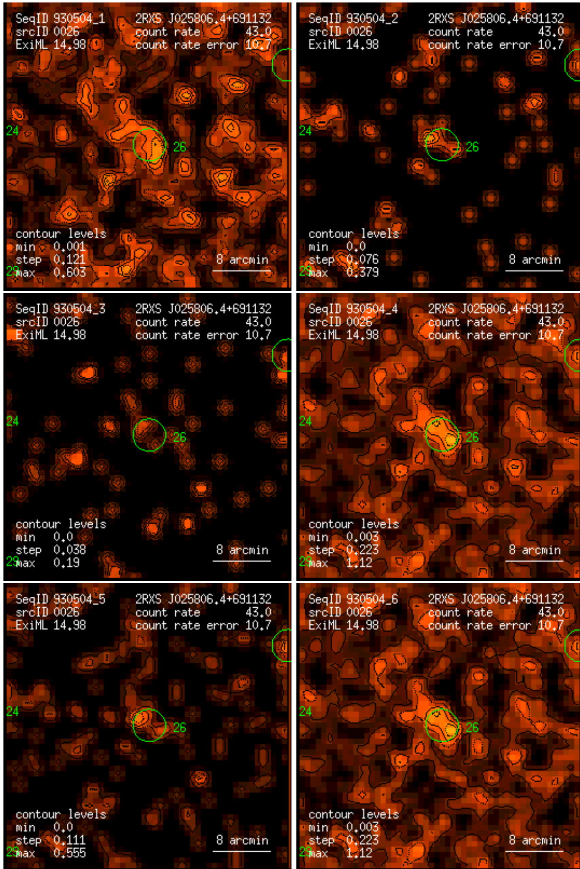
Figure 26: RASS 930504: detection 0026: band rate images, Gaussian filter: (1) PSPC channels 11 – 41, (2) 52 – 90, (3) 91 – 201, (4) 11 – 235, (5) 52 – 201, (6) 11 – 201. Broad band rates in counts/ks. Band rate contour levels in counts/ks/arcmin 2 .
