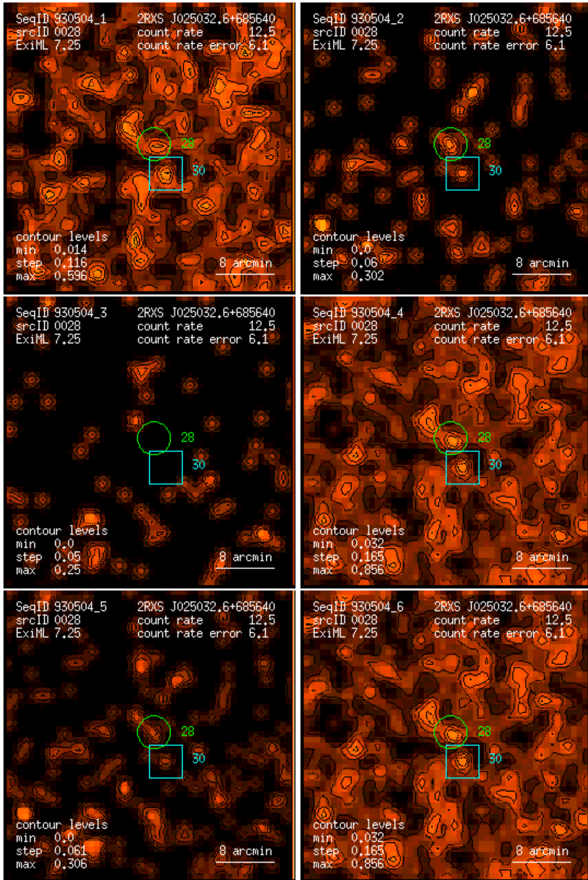
Figure 28: RASS 930504: detection 0028: band rate images, Gaussian filter: (1) PSPC channels 11 – 41, (2) 52 – 90, (3) 91 – 201, (4) 11 – 235, (5) 52 – 201, (6) 11 – 201. Broad band rates in counts/ks. Band rate contour levels in counts/ks/arcmin 2 .
