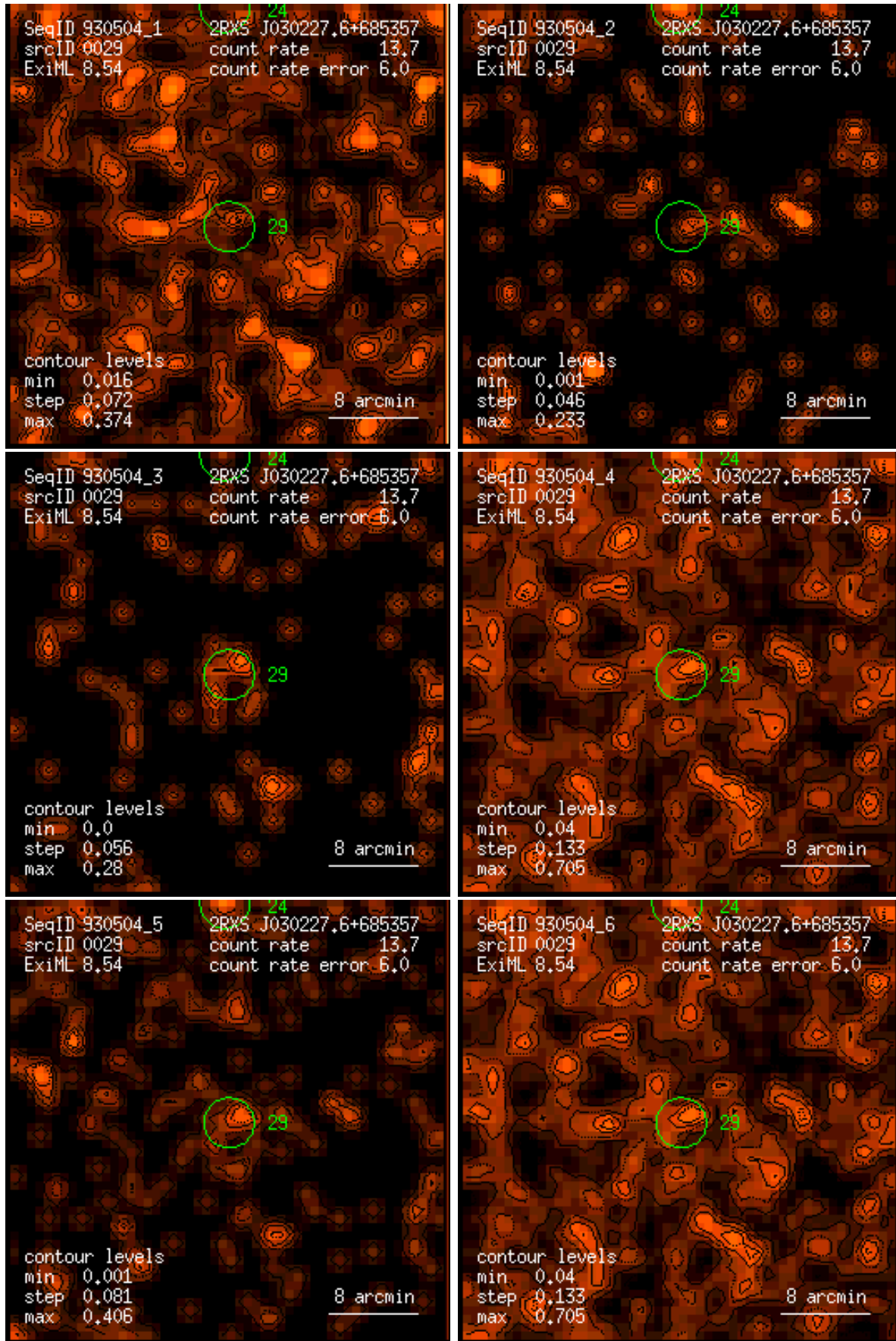
Figure 29: RASS 930504: detection 0029: band rate images, Gaussian filter: (1) PSPC channels 11 – 41, (2) 52 – 90, (3) 91 – 201, (4) 11 – 235, (5) 52 – 201, (6) 11 – 201. Broad band rates in counts/ks. Band rate contour levels in counts/ks/arcmin 2 .
