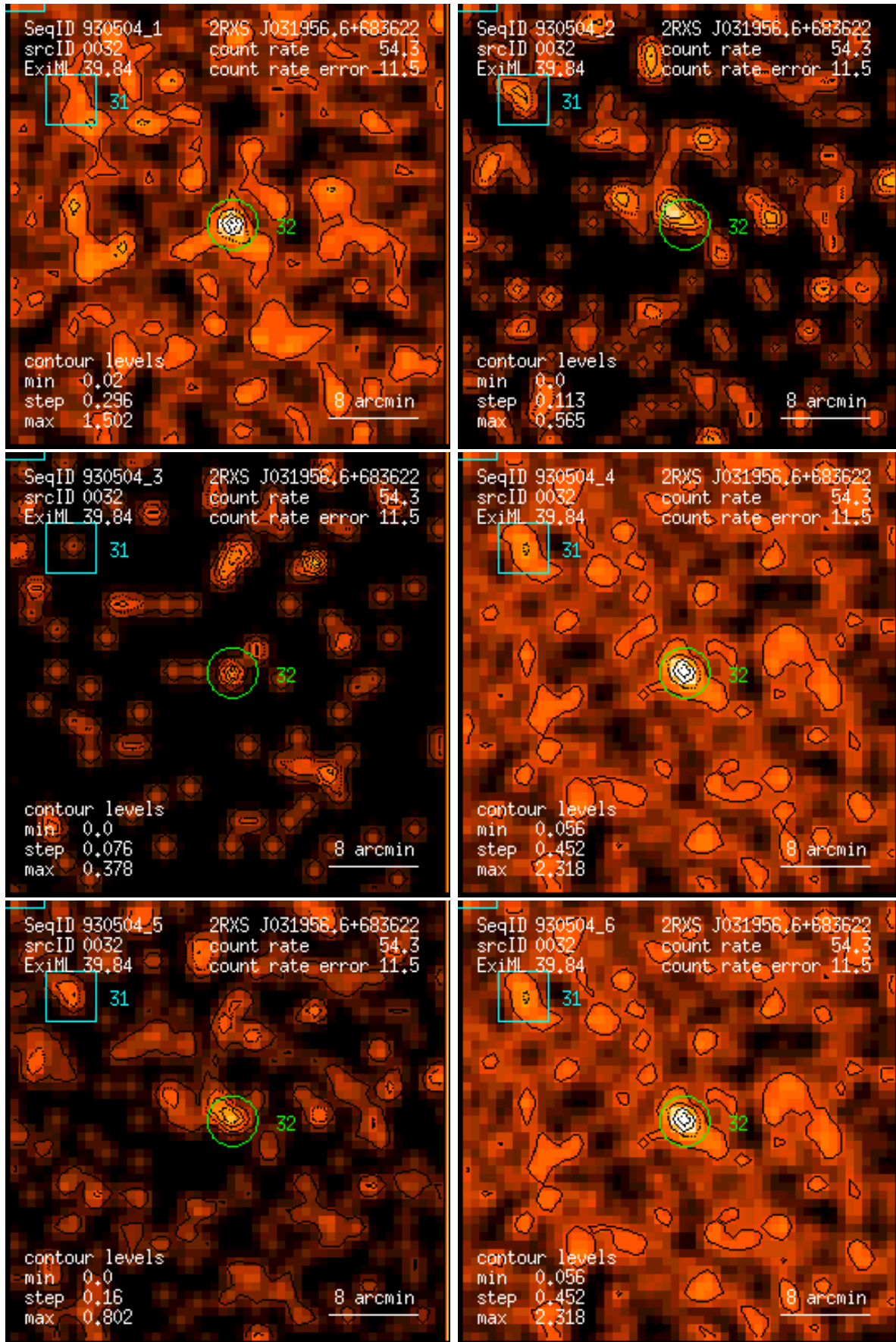
Figure 32: RASS 930504: detection 0032: band rate images, Gaussian filter: (1) PSPC channels 11 – 41, (2) 52 – 90, (3) 91 – 201, (4) 11 – 235, (5) 52 – 201, (6) 11 – 201. Broad band rates in counts/ks. Band rate contour levels in counts/ks/arcmin 2 .
