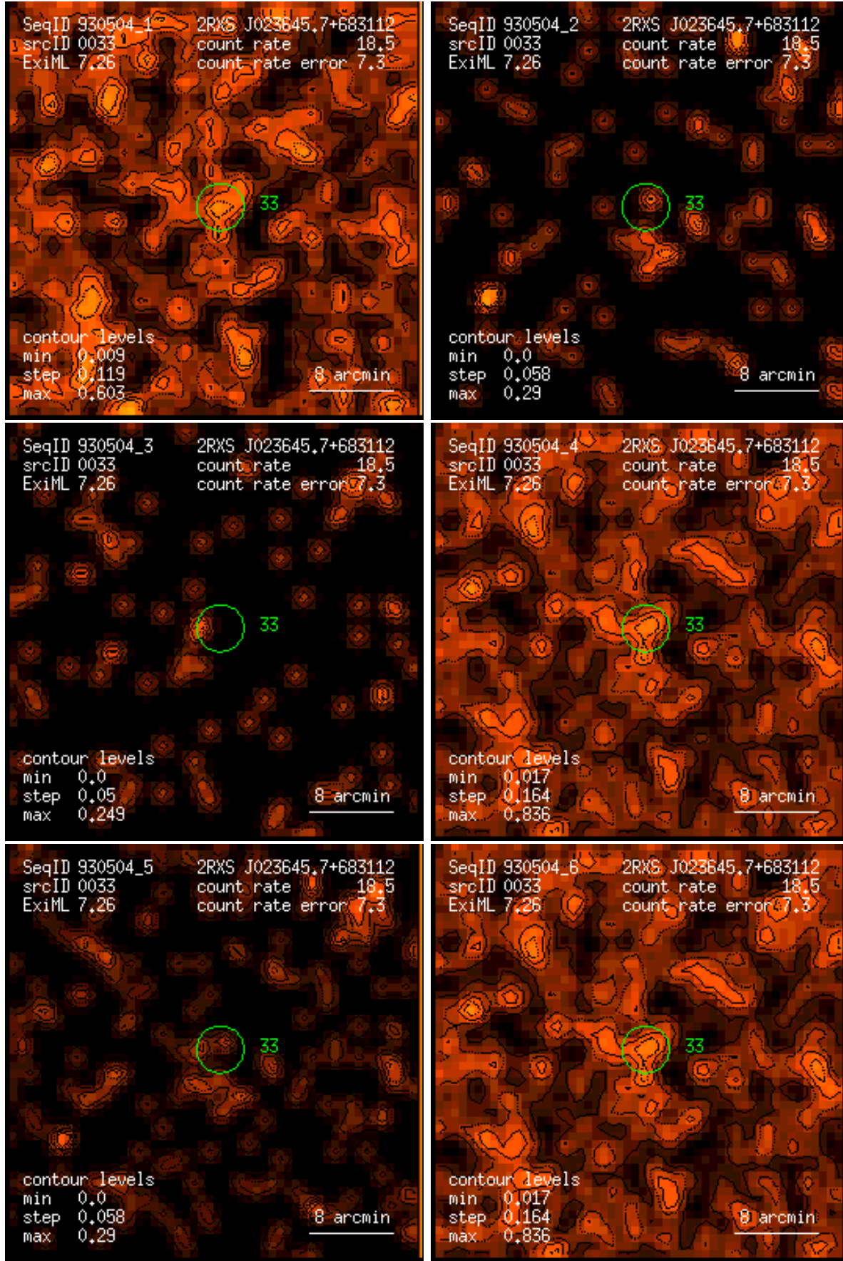
Figure 33: RASS 930504: detection 0033: band rate images, Gaussian filter: (1) PSPC channels 11 – 41, (2) 52 – 90, (3) 91 – 201, (4) 11 – 235, (5) 52 – 201, (6) 11 – 201. Broad band rates in counts/ks. Band rate contour levels in counts/ks/arcmin 2 .
