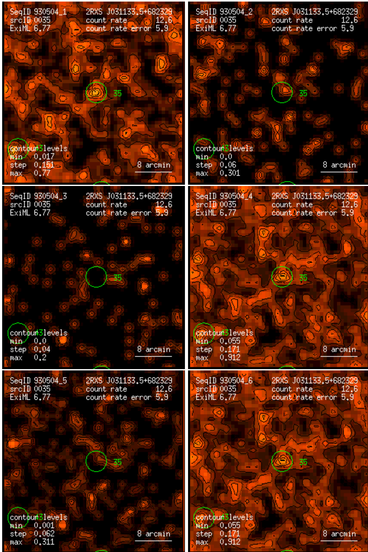
Figure 35: RASS 930504: detection 0035: band rate images, Gaussian filter: (1) PSPC channels 11 – 41, (2) 52 – 90, (3) 91 – 201, (4) 11 – 235, (5) 52 – 201, (6) 11 – 201. Broad band rates in counts/ks. Band rate contour levels in counts/ks/arcmin 2 .
