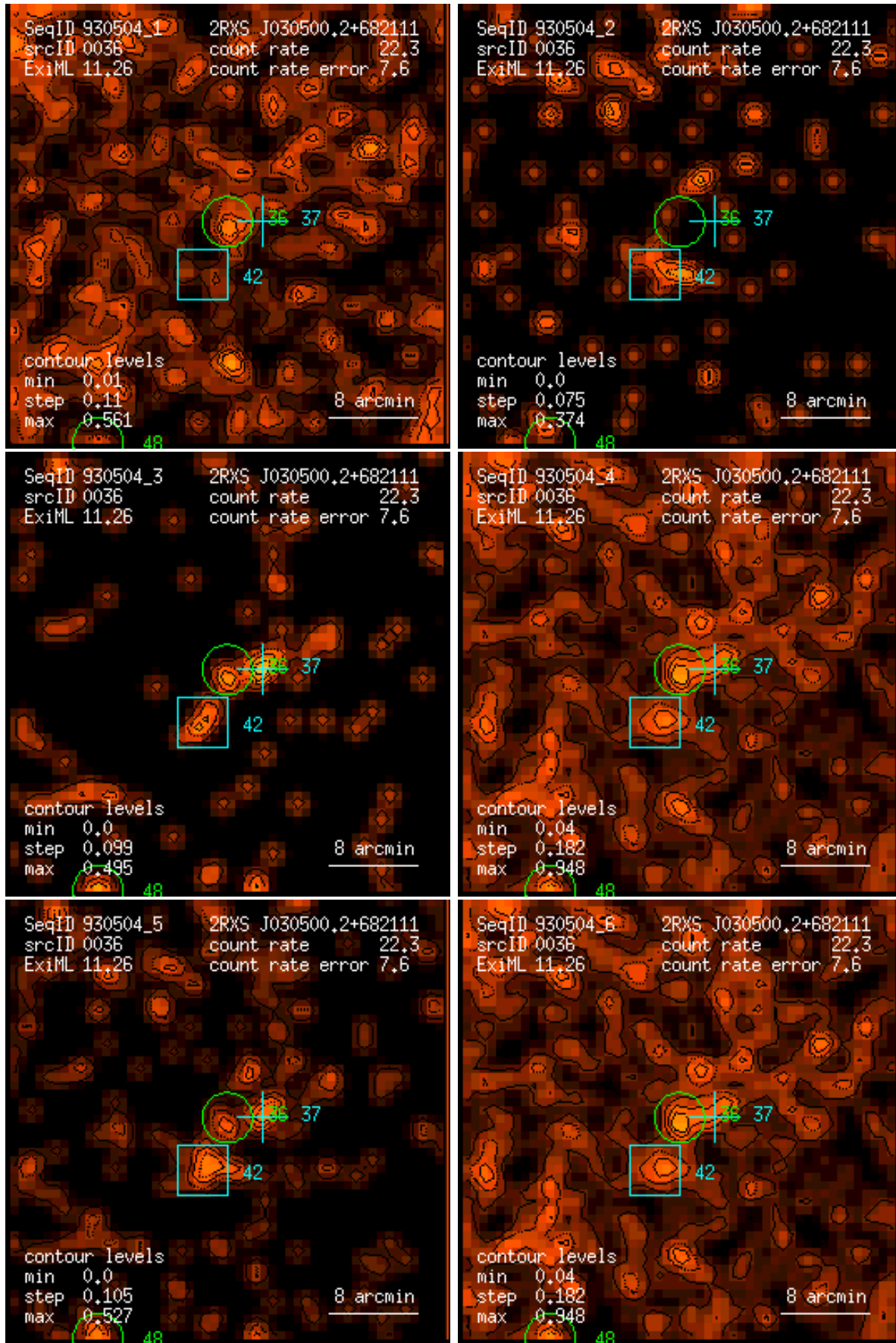
Figure 36: RASS 930504: detection 0036: band rate images, Gaussian filter: (1) PSPC channels 11 – 41, (2) 52 – 90, (3) 91 – 201, (4) 11 – 235, (5) 52 – 201, (6) 11 – 201. Broad band rates in counts/ks. Band rate contour levels in counts/ks/arcmin 2 .
