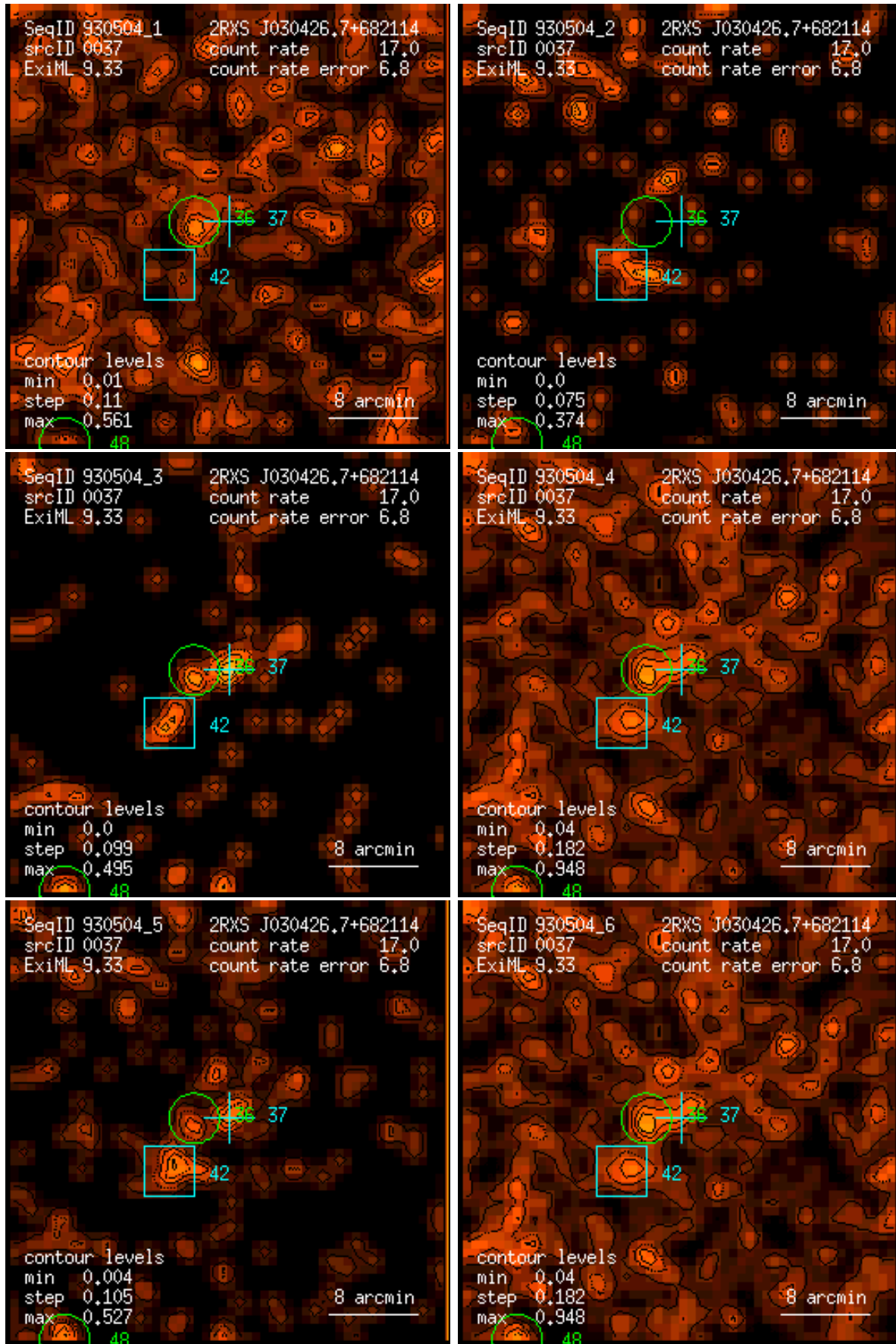
Figure 37: RASS 930504: detection 0037: band rate images, Gaussian filter: (1) PSPC channels 11 – 41, (2) 52 – 90, (3) 91 – 201, (4) 11 – 235, (5) 52 – 201, (6) 11 – 201. Broad band rates in counts/ks. Band rate contour levels in counts/ks/arcmin 2 .
