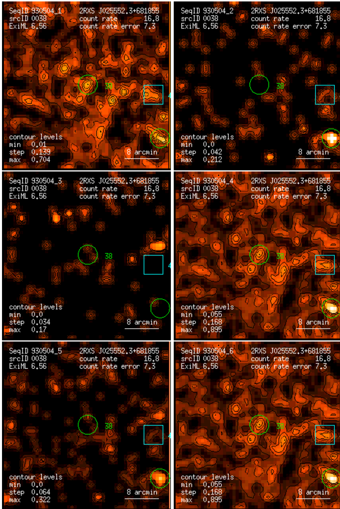
Figure 38: RASS 930504: detection 0038: band rate images, Gaussian filter: (1) PSPC channels 11 – 41, (2) 52 – 90, (3) 91 – 201, (4) 11 – 235, (5) 52 – 201, (6) 11 – 201. Broad band rates in counts/ks. Band rate contour levels in counts/ks/arcmin 2 .
