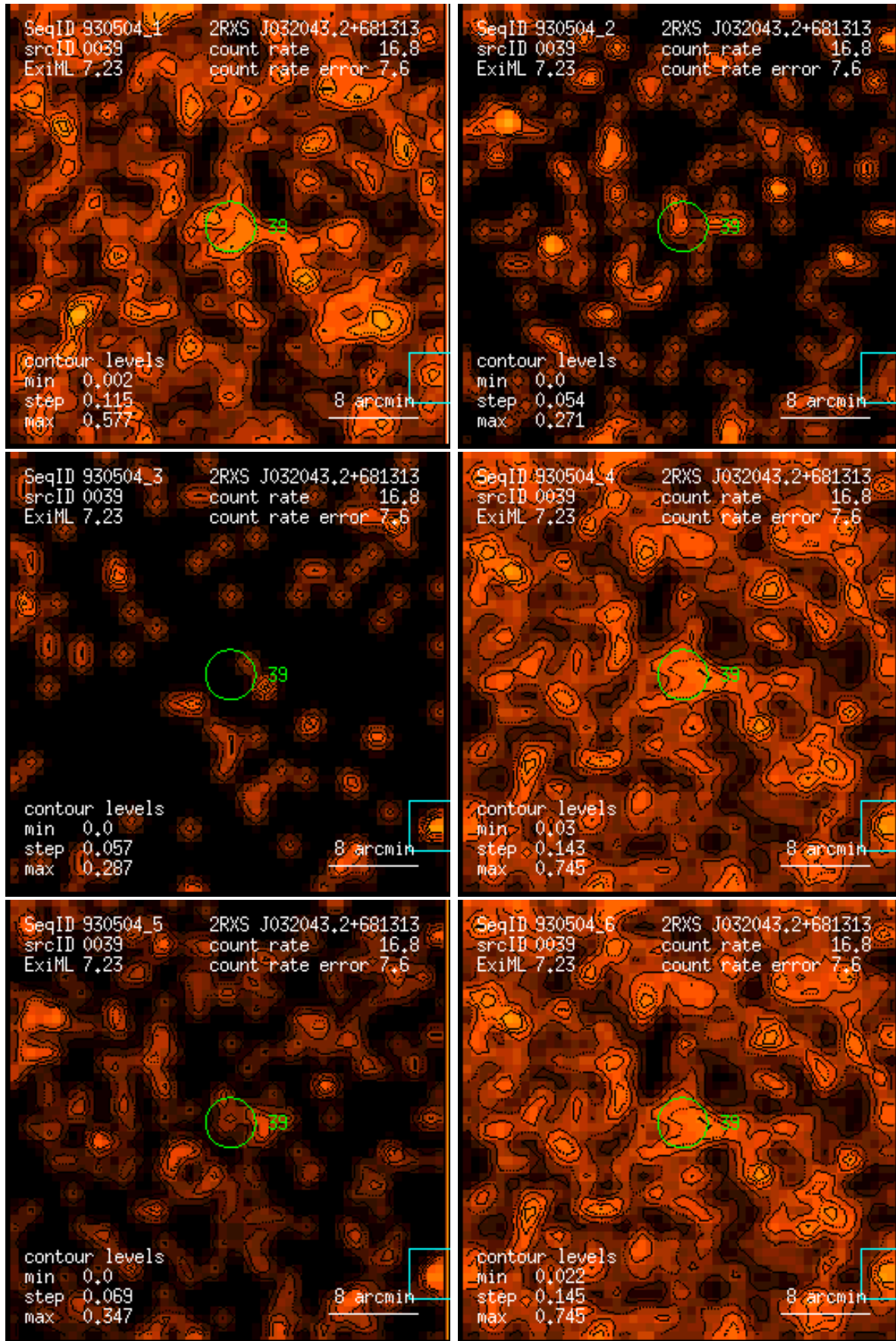
Figure 39: RASS 930504: detection 0039: band rate images, Gaussian filter: (1) PSPC channels 11 – 41, (2) 52 – 90, (3) 91 – 201, (4) 11 – 235, (5) 52 – 201, (6) 11 – 201. Broad band rates in counts/ks. Band rate contour levels in counts/ks/arcmin 2 .
