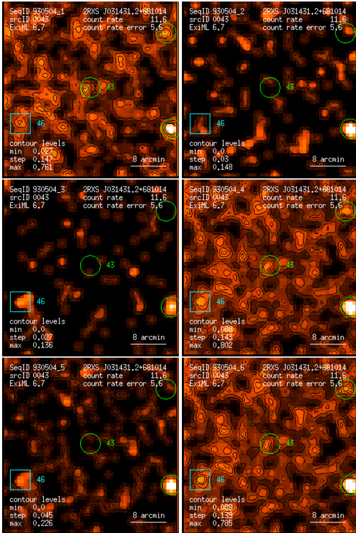
Figure 43: RASS 930504: detection 0043: band rate images, Gaussian filter: (1) PSPC channels 11 – 41, (2) 52 – 90, (3) 91 – 201, (4) 11 – 235, (5) 52 – 201, (6) 11 – 201. Broad band rates in counts/ks. Band rate contour levels in counts/ks/arcmin 2 .
