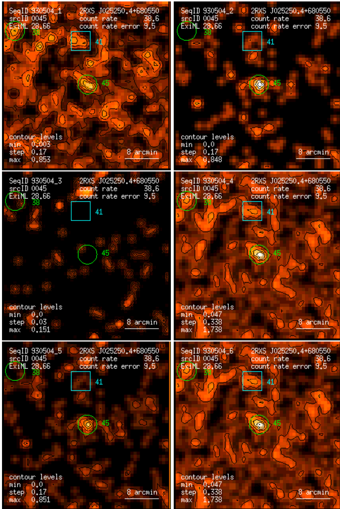
Figure 45: RASS 930504: detection 0045: band rate images, Gaussian filter: (1) PSPC channels 11 – 41, (2) 52 – 90, (3) 91 – 201, (4) 11 – 235, (5) 52 – 201, (6) 11 – 201. Broad band rates in counts/ks. Band rate contour levels in counts/ks/arcmin 2 .
