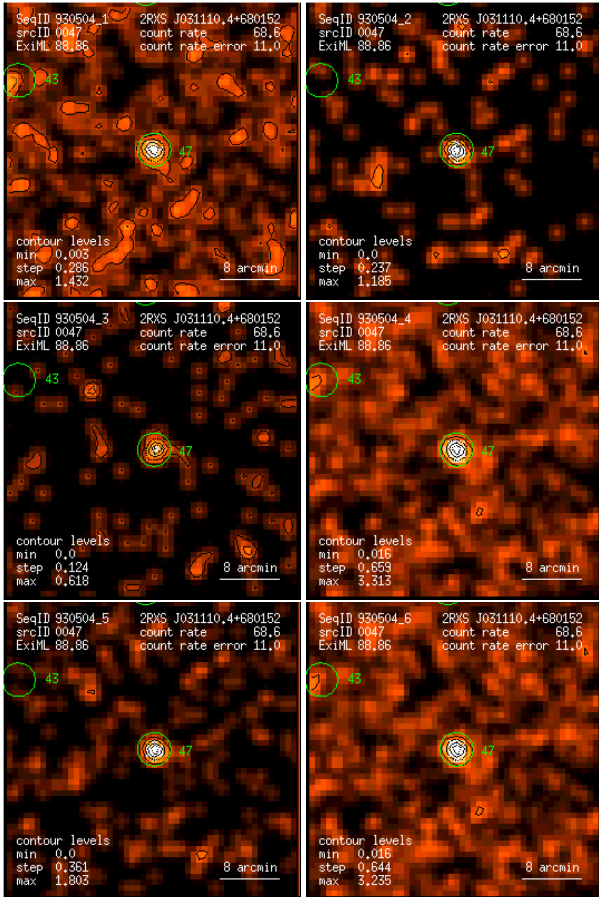
Figure 47: RASS 930504: detection 0047: band rate images, Gaussian filter: (1) PSPC channels 11 – 41, (2) 52 – 90, (3) 91 – 201, (4) 11 – 235, (5) 52 – 201, (6) 11 – 201. Broad band rates in counts/ks. Band rate contour levels in counts/ks/arcmin 2 .
