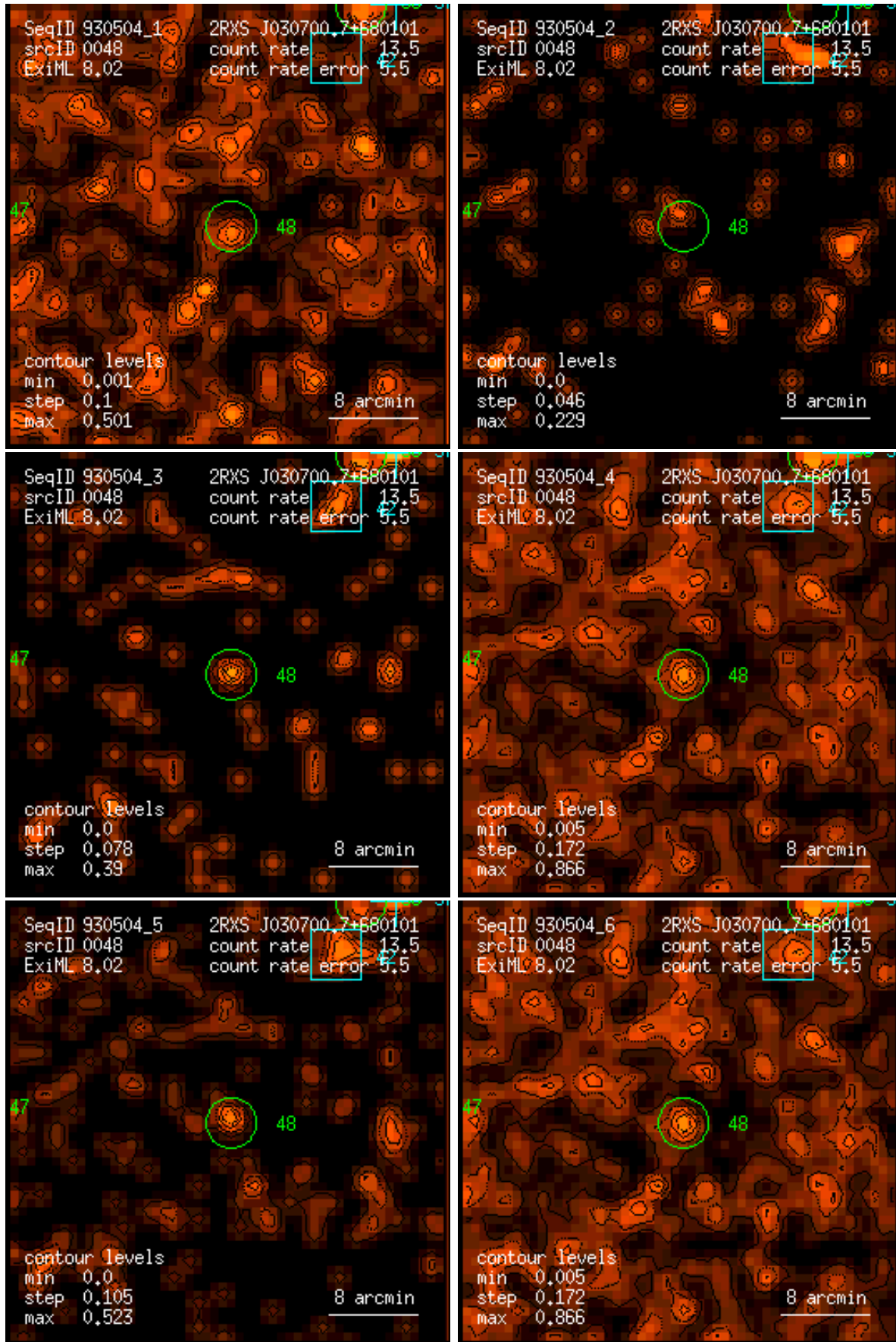
Figure 48: RASS 930504: detection 0048: band rate images, Gaussian filter: (1) PSPC channels 11 – 41, (2) 52 – 90, (3) 91 – 201, (4) 11 – 235, (5) 52 – 201, (6) 11 – 201. Broad band rates in counts/ks. Band rate contour levels in counts/ks/arcmin 2 .
