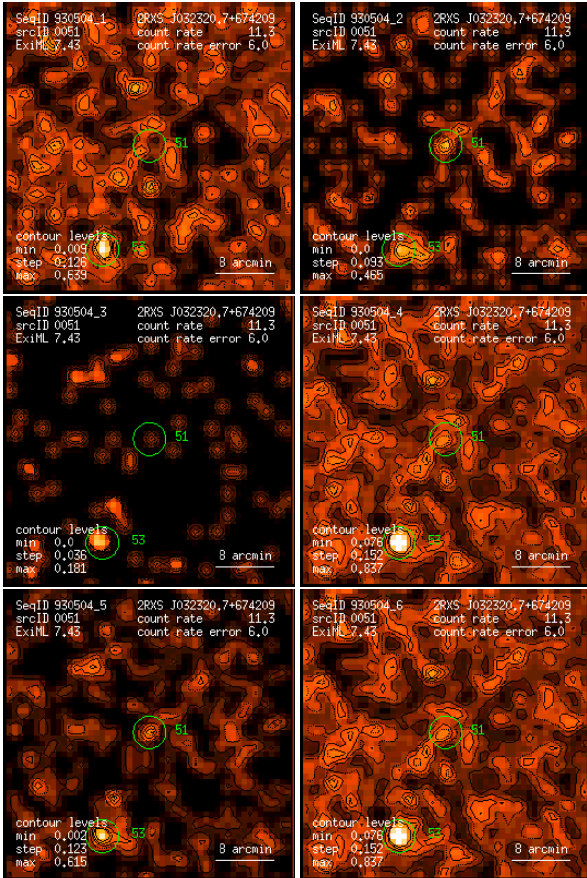
Figure 51: RASS 930504: detection 0051: band rate images, Gaussian filter: (1) PSPC channels 11 – 41, (2) 52 – 90, (3) 91 – 201, (4) 11 – 235, (5) 52 – 201, (6) 11 – 201. Broad band rates in counts/ks. Band rate contour levels in counts/ks/arcmin 2 .
