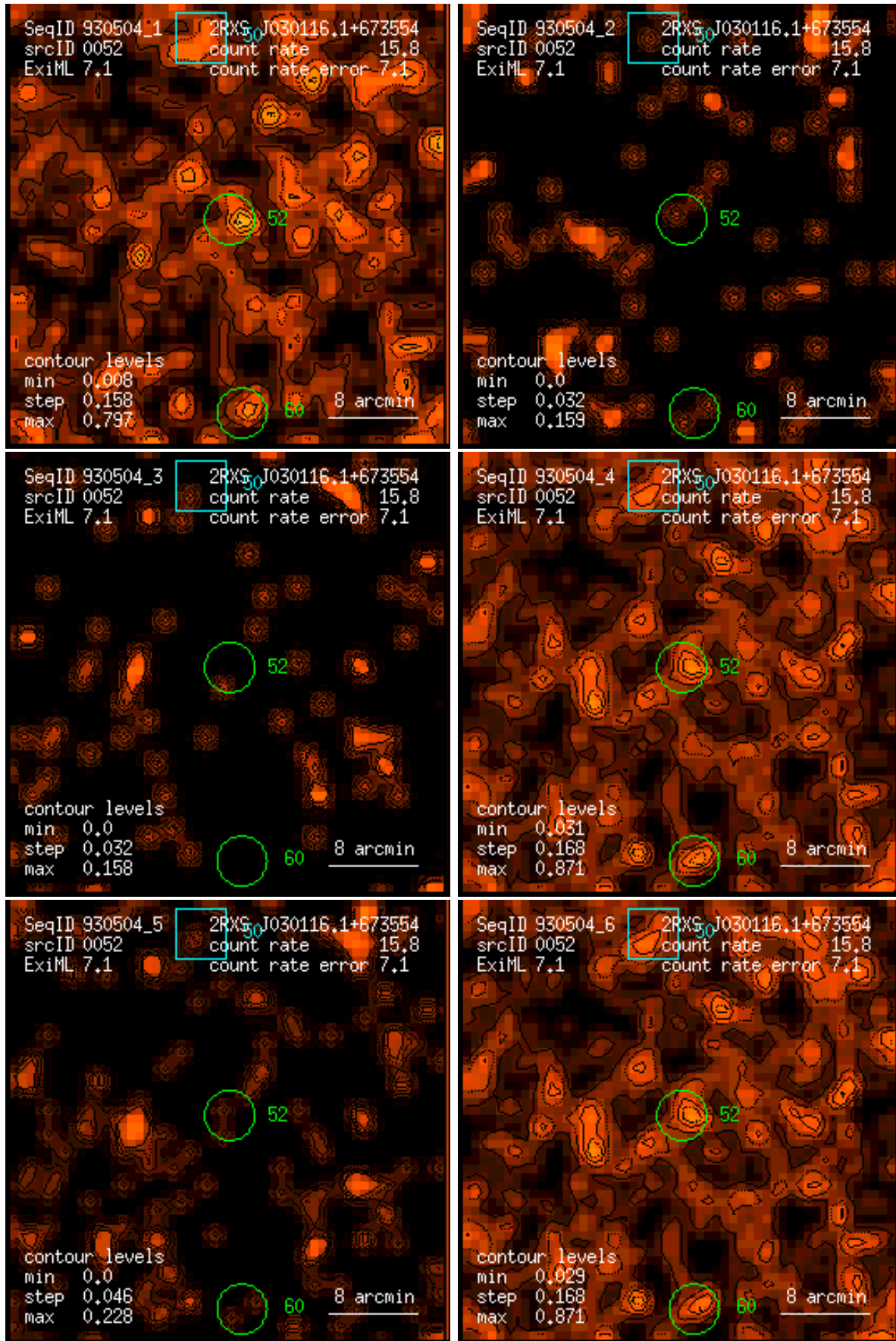
Figure 52: RASS 930504: detection 0052: band rate images, Gaussian filter: (1) PSPC channels 11 – 41, (2) 52 – 90, (3) 91 – 201, (4) 11 – 235, (5) 52 – 201, (6) 11 – 201. Broad band rates in counts/ks. Band rate contour levels in counts/ks/arcmin 2 .
