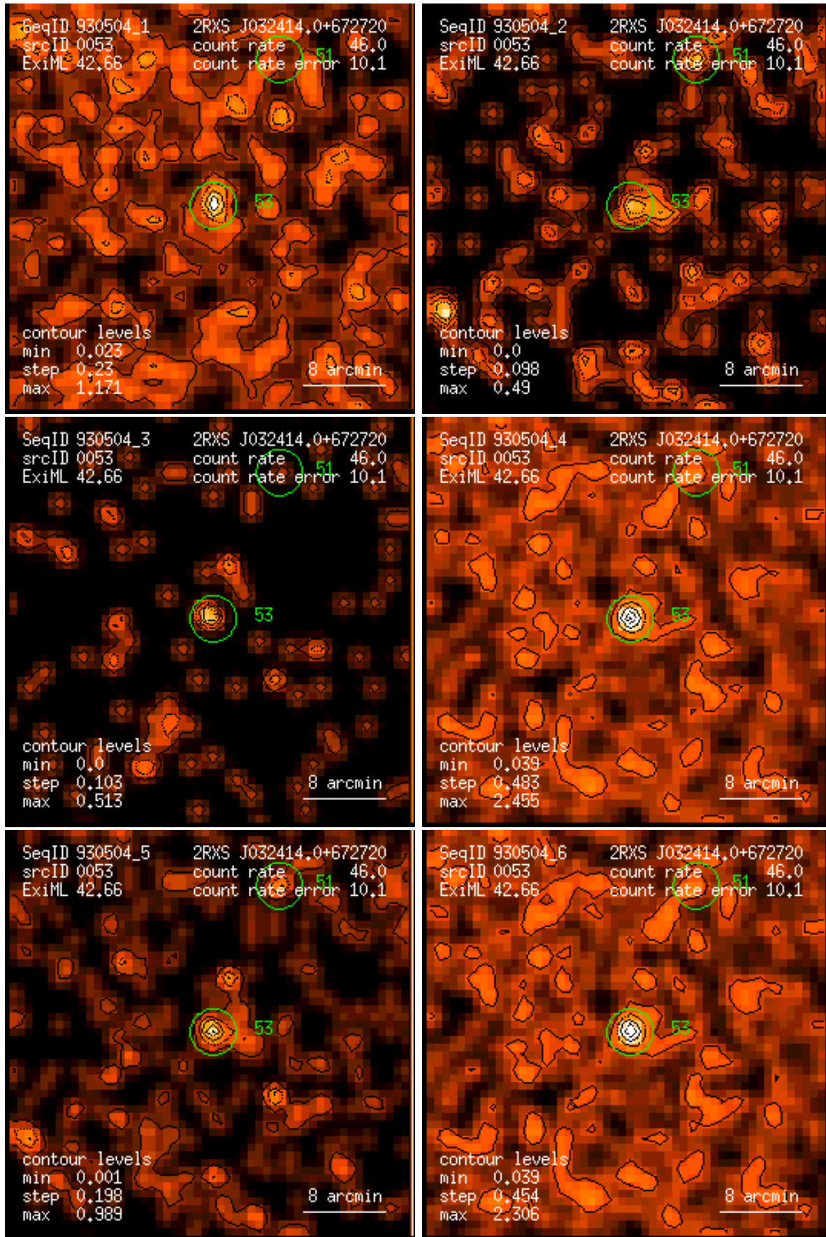
Figure 53: RASS 930504: detection 0053: band rate images, Gaussian filter: (1) PSPC channels 11 – 41, (2) 52 – 90, (3) 91 – 201, (4) 11 – 235, (5) 52 – 201, (6) 11 – 201. Broad band rates in counts/ks. Band rate contour levels in counts/ks/arcmin 2 .
