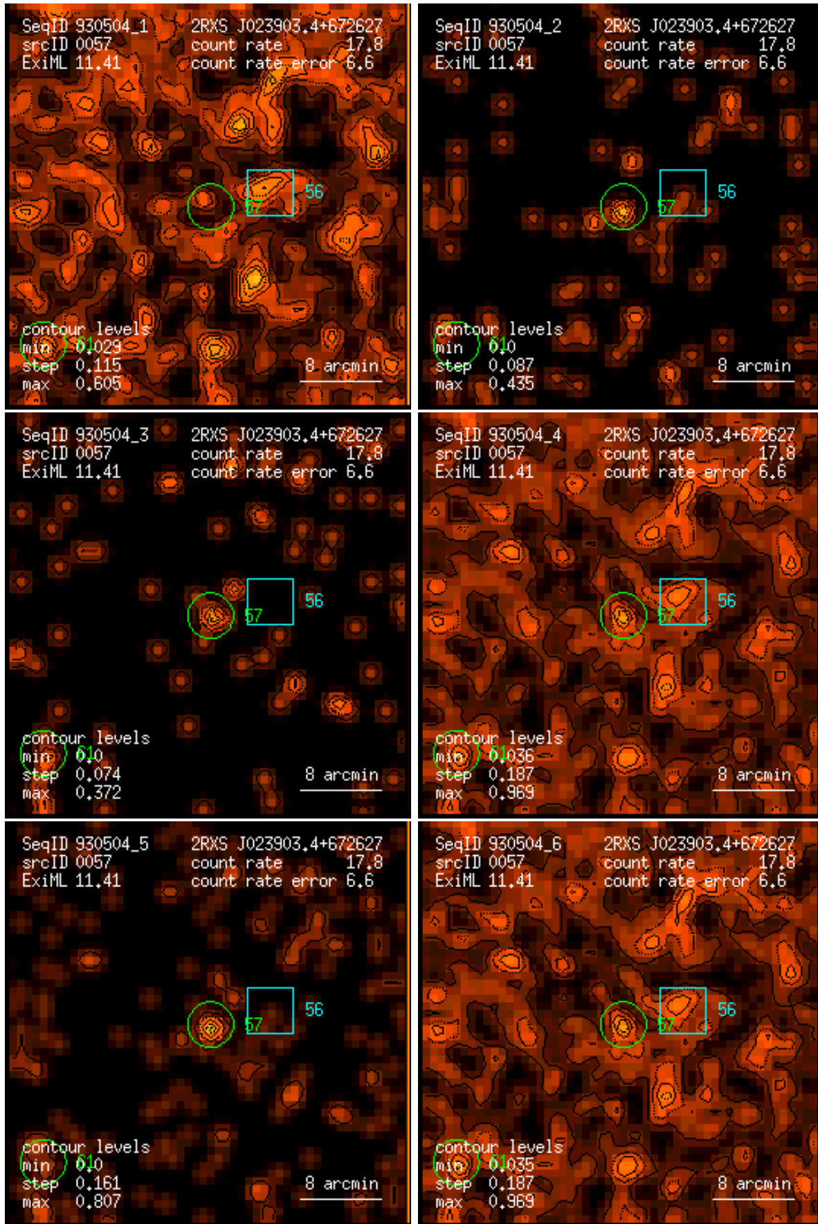
Figure 57: RASS 930504: detection 0057: band rate images, Gaussian filter: (1) PSPC channels 11 – 41, (2) 52 – 90, (3) 91 – 201, (4) 11 – 235, (5) 52 – 201, (6) 11 – 201. Broad band rates in counts/ks. Band rate contour levels in counts/ks/arcmin 2 .
