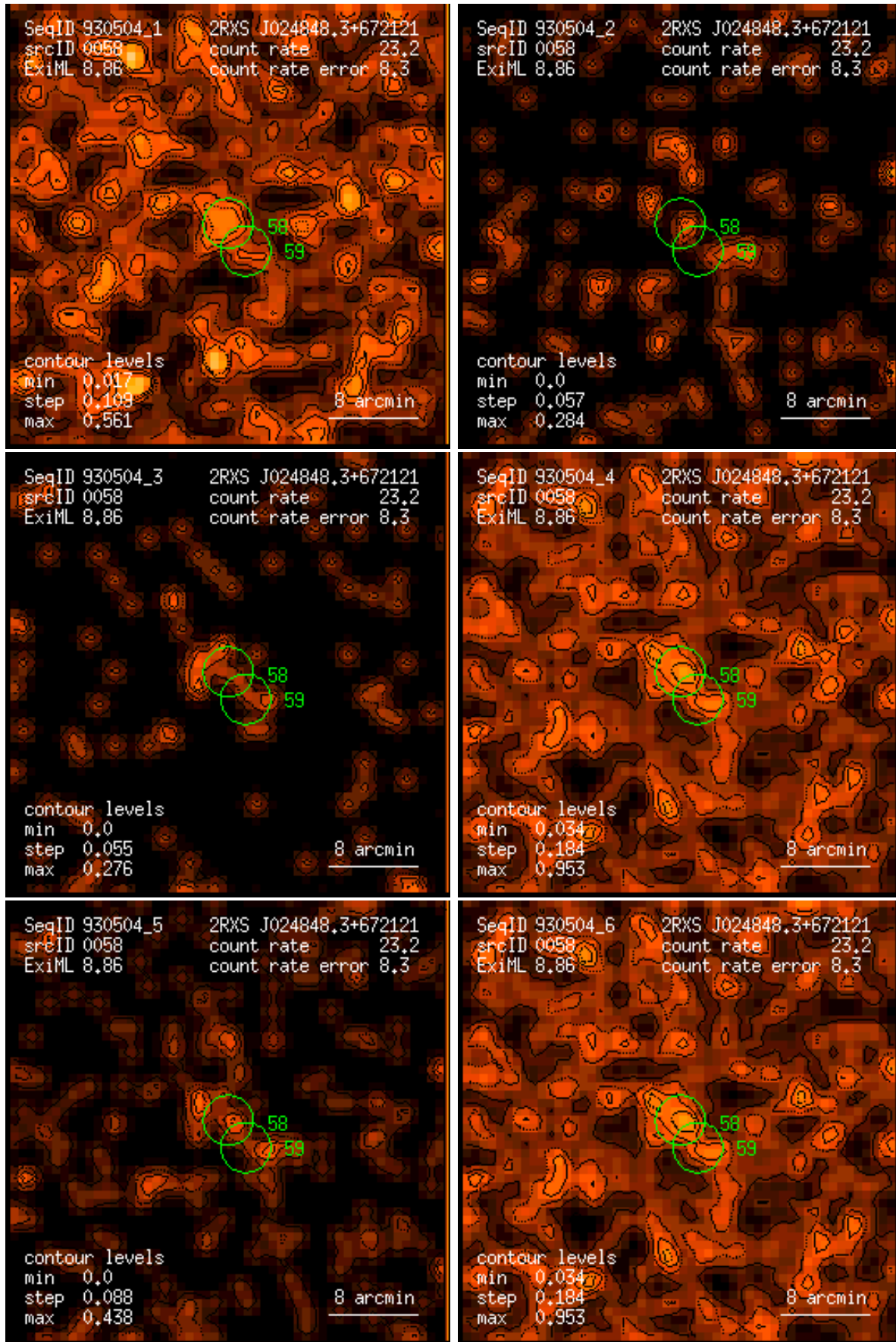
Figure 58: RASS 930504: detection 0058: band rate images, Gaussian filter: (1) PSPC channels 11 – 41, (2) 52 – 90, (3) 91 – 201, (4) 11 – 235, (5) 52 – 201, (6) 11 – 201. Broad band rates in counts/ks. Band rate contour levels in counts/ks/arcmin 2 .
