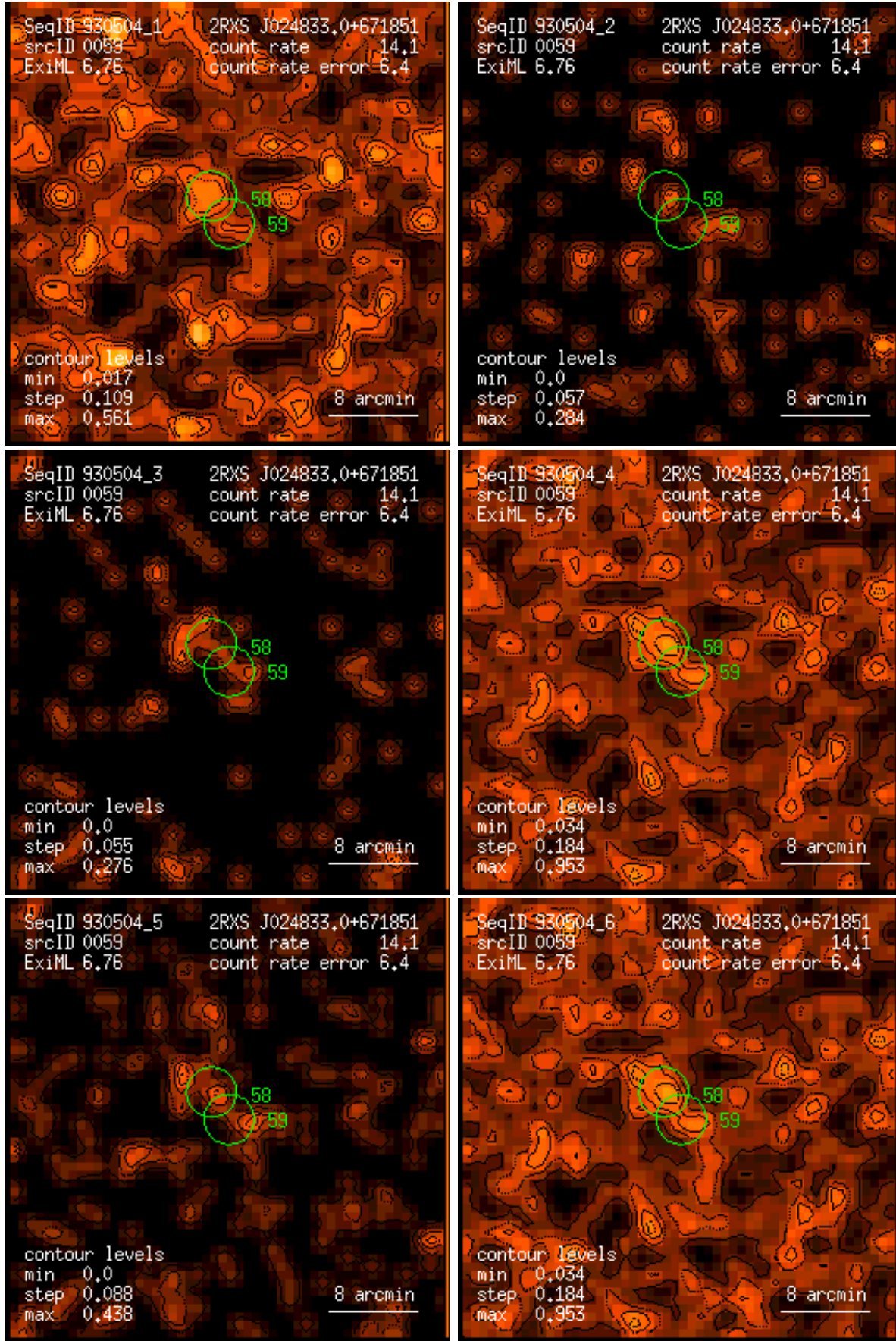
Figure 59: RASS 930504: detection 0059: band rate images, Gaussian filter: (1) PSPC channels 11 – 41, (2) 52 – 90, (3) 91 – 201, (4) 11 – 235, (5) 52 – 201, (6) 11 – 201. Broad band rates in counts/ks. Band rate contour levels in counts/ks/arcmin 2 .
