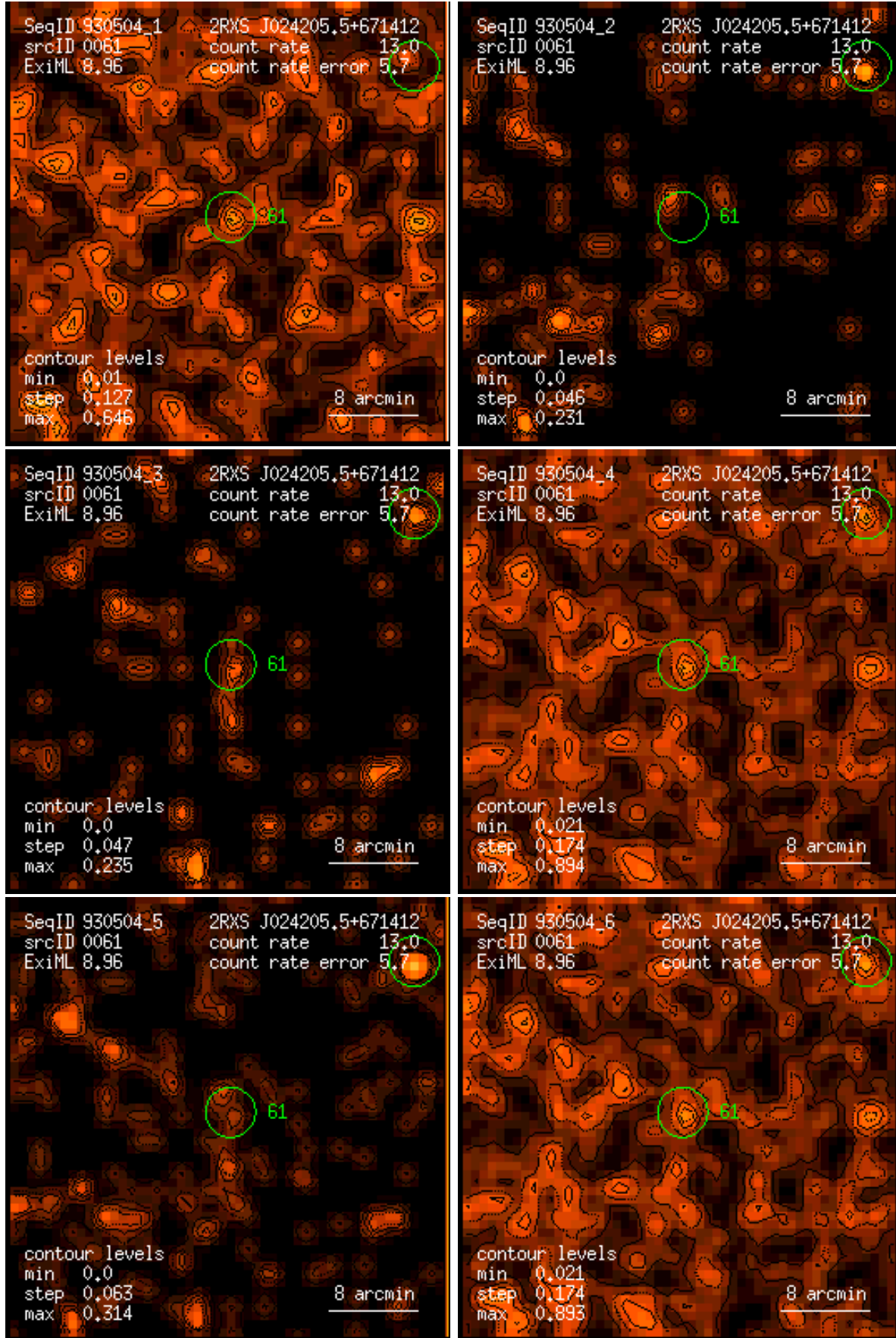
Figure 61: RASS 930504: detection 0061: band rate images, Gaussian filter: (1) PSPC channels 11 – 41, (2) 52 – 90, (3) 91 – 201, (4) 11 – 235, (5) 52 – 201, (6) 11 – 201. Broad band rates in counts/ks. Band rate contour levels in counts/ks/arcmin 2 .
